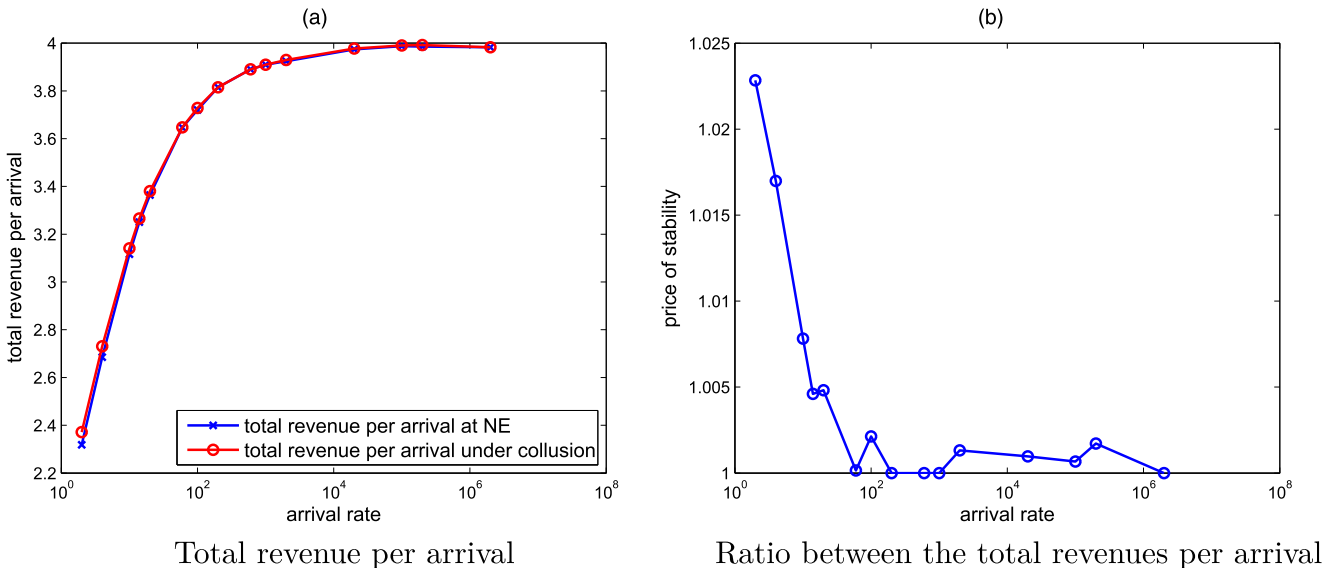
Figure 3. Total Revenue per Arrival in Nash Equilibrium and Under Collusion and Their Ratio When V = 5
