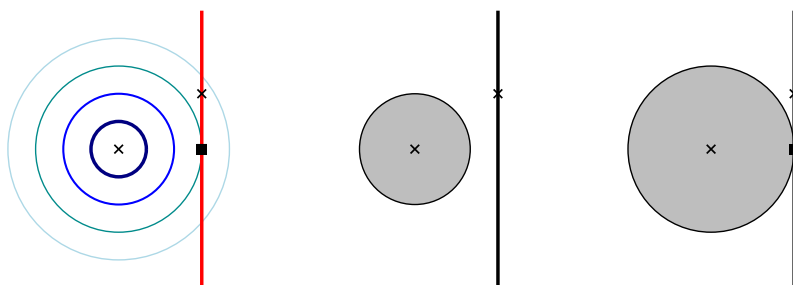
FIG. 6. Example of DCPs. This is a d = 2 case; there is a 2D spherical distribution mixed with a 1D distribution on a line segment. Left: the blue contours are density contours of the 2D spherical distribution and the red line segment is \mathbb{K}_1 , the support of the 1D singular distribution. The two crosses are the density maxima at the 2D distribution and the 1D singular distribution. The black square indicates a DCP. To see how DCPs merge two connected components, we consider the middle and the right panel, which are level sets of \alpha(x) at two different levels. Middle: the level set \mathbb{A}_{\varpi} where the level \varpi is high; we can see that there are two connected components (left gray-black disk and the right line segment). Right: we move down the level a little bit; now the two connected components merge so there is only one connected component. The merging point is the square point, which is defined as a DCP.
