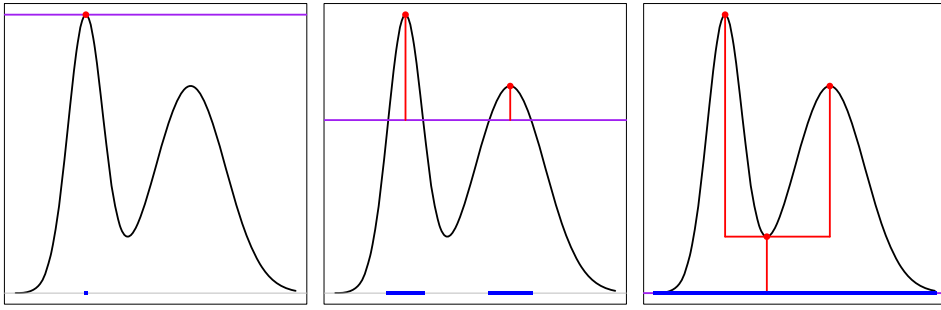
FIG. 1. An example of constructing a cluster tree in d = 1 case. The purple horizontal lines indicates the level f_0 we are using in each panel. The blue region at the bottom indicates the corresponding level set \{x : f(x) \geq f_0\} . From left to right, we gradually decrease the level f_0 and use red lines to indicate how the connected components evolve. The resulting red tree in the right panel is a cluster tree.
