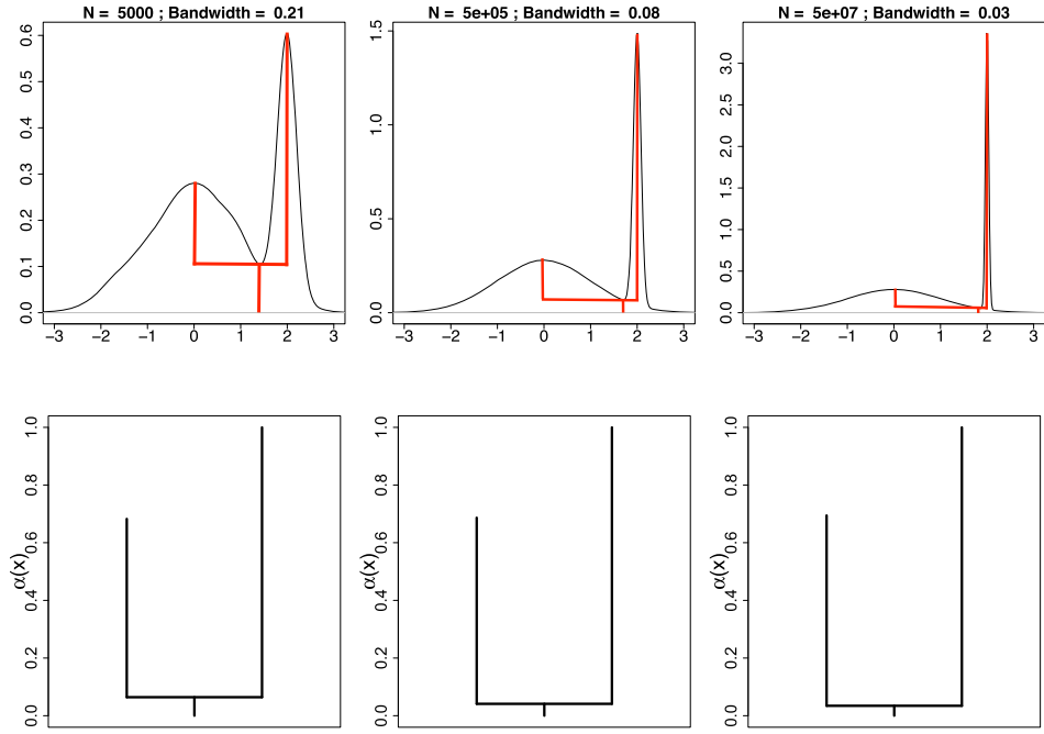
FIG. 2. Example of the estimated \lambda -tree and \alpha -tree of a singular distribution. This is a random sample from a singular distribution where with a probability of 0.3, it puts a point mass at x = 2 , and with a probability of 0.7, we sample from a standard normal. The top panel shows the density estimated by the KDE and the red tree structure corresponds to the estimated \lambda -tree. The bottom panel displays the estimated \alpha -tree. From left to right, we increase the sample size from 5 \times 10^3 , 5 \times 10^5 , to 5 \times 10^7 . Because the distribution is singular, there is no population \lambda -tree so when the smoothing bandwidth decreases (when the sample size increases), the estimated \lambda -tree is getting degenerated. On the other hand, the estimated \alpha -trees remain stable regardless of the smoothing bandwidth. Note that every level set in a \lambda -tree corresponds to a level set in the \alpha -tree but the value of the corresponding level (Y-axis) will be different. The function used in constructing a \lambda -tree may have an unbounded range when the sample size goes to infinity, whereas the function for building an \alpha -tree always has a range of [0, 1] .
