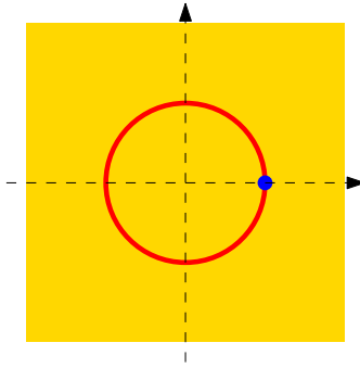
FIG. 4. The supports \mathbb{K}_2 , \mathbb{K}_1 , and \mathbb{K}_0 for the bivariate random variable in Example 1. The yellow region is \mathbb{K}_2 = [-1, 1]^2 \setminus R_{0.5} , where R_{0.5} = \{(x, y) : x^2 + y^2 = 0.5^2\} . The red ring is \mathbb{K}_1 = R_{0.5} \setminus \{(0.5, 0)\} . The blue dot is the location of (0.5, 0) .
