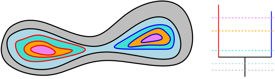
FIG. 3. Connected components, edges, and edge set of a cluster tree. Left: We display connected components of level sets under five different levels (indicated by the colors: magenta, yellow, sea green, sky blue and gray). The color of boundaries of each connected component denotes the edge they correspond to. Right: The cluster tree. We color the three edges (vertical lines) red, blue and black. The edge set E(T_f) = \{\mathbb{C}_{\text{red}}, \mathbb{C}_{\text{blue}}, \mathbb{C}_{\text{black}}\} and we have the ordering \mathbb{C}_{\text{red}} \leq \mathbb{C}_{\text{black}} and \mathbb{C}_{\text{blue}} \leq \mathbb{C}_{\text{black}} . Note that the solid black horizontal line is not an edge set; it is a visual representation of connecting the blue and red edges to the black edge. The horizontal dashed lines indicate the five levels corresponding to the left panel. In the left panel, the three connected components with red boundaries are elements of the edge \mathbb{C}_{\text{red}} .
