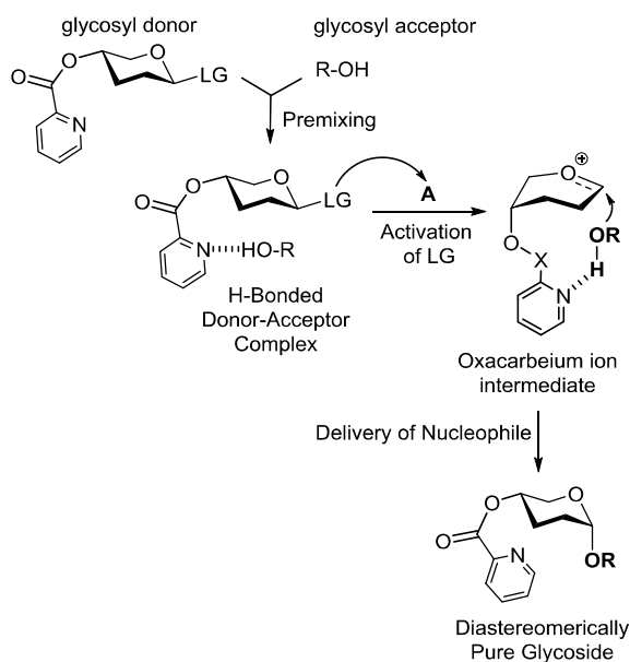
Scheme 1. Mechanistic depiction of the HAD glycosylation method.
