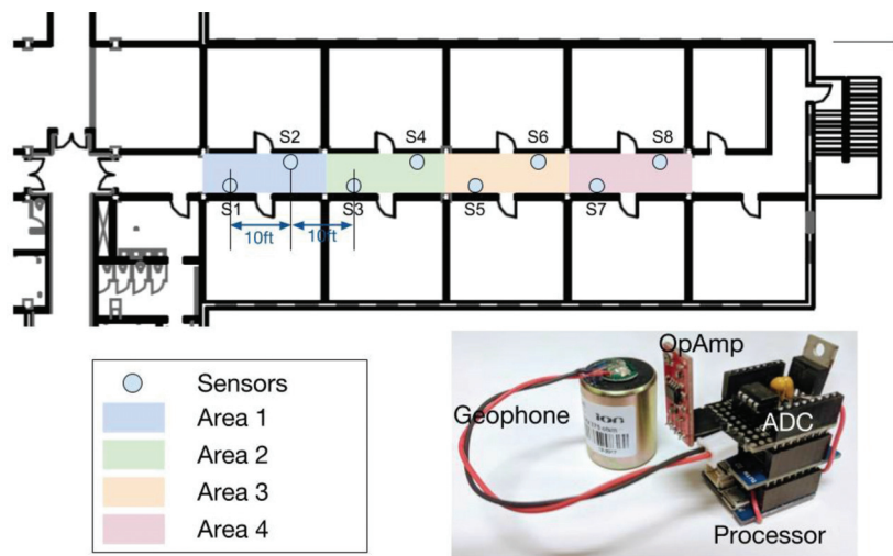
Figure 3. Sensor deployment and the floor plan. Lower right image shows the sensing node utilized for the uncontrolled experiments.
