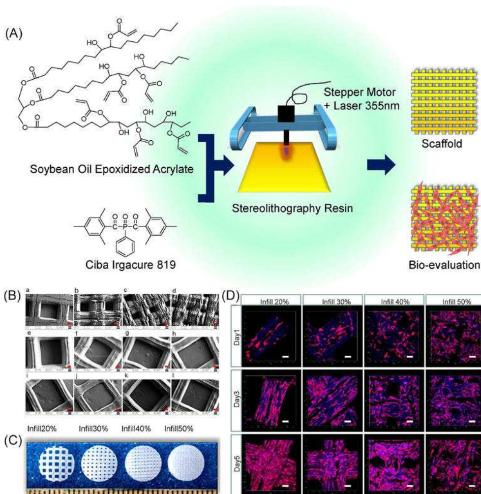
Figure 5. (A) Schematic of soybean oil epoxidized acrylate fabrication process from raw material through resin fabrication and application. (B) SEM images of printed scaffolds, red scale bar 100 \mu\text{m} . (a–d) Printing speed 10 mm/s, laser frequency 20,000 Hz, infill density 20%, 30%, 40% and 50%, respectively; (e–j) Laser frequency 12,000 Hz, infill density 20%, printing speeds 10, 20, 30, 40, 60, and 80 mm/s, respectively; (k and l) Infill density 20%, printing speed 10 mm/s, laser intensity 16,000 and 8000 Hz, respectively. (C) Confocal images of hMSCs spreading on printed scaffolds from soybean oil epoxidized acrylate (printing speed 10 mm/s, laser frequency 20,000 Hz) with different infill density. Data are mean \pm standard deviation, n = 6 . * p < 0.05 , ** p < 0.01 , *** p < 0.001 . Scale bars are 100 \mu\text{m} .
