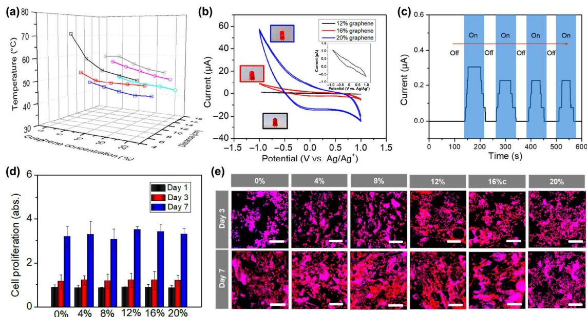
Figure 5 Characterization of NIR sensitive 4D printed constructs. (a) Effect of the parameters of NIR laser and material component on the 4D transformation process, including different graphene content, exposure distance, and laser intensity. \square represents 800 mW NIR illumination, \circ represents 1,800 mW NIR illumination; line colors show different exposure distances (— 6 cm, — 8 cm, — 10 cm, — 14 cm, — 16 cm, and — 18 cm). (b) Cyclic voltammogram curves of different nanocomposites doped with 12%, 16%, and 20% graphene. The inset curve shows nanocomposite with 12% graphene. The inset images illustrate different brightness of the lamp, where the blue frame shows 20% sample, red frame shows 16% sample, and the black frame shows 12% sample, indicating good electroconductivity of the samples. (c) Optoelectrical property of the nanocomposites with 16% graphene. When the light is on, a slight photocurrent can be detected; after the light is turned off, the photocurrent disappears. (d) NSC proliferation on different 4D printed samples after 1, 3, and 7 days of culture. (e) NSC morphology on different 4D printed samples after 3 and 7 days of culture, where F-actin is colored red and nucleus is colored blue. Scale bar is 200 \mu m. There is no significant difference among these samples (N.S.), suggesting graphene doped nanocomposites exhibited an excellent cytocompatibility in vitro .
