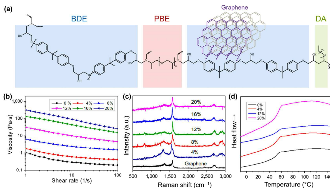
Figure 1 Synthesis and characterization of 4D nanocomposite inks. (a) Chemical structures of the nanocomposite ink consisted of the thermally responsive SMP and photothermally responsive graphene. Dotted lines show the \pi - \pi interaction between SMP and graphene. The SMP includes three segments: a rigid epoxy monomer (bisphenol A diglycidyl ether, BDE), an aliphatic diamine crosslinker (poly(propylene glycol) bis(2-aminopropyl) ether, PBE), and a crosslinking modulator (decylamine, DA, which is used to tailor the T_g of the polymers). (b) Dynamic viscosity of 4D nanocomposite inks measured by rheometer at room temperature. It shows a typical shear thinning behavior, and the viscosity of the inks increase with increasing graphene content. (c) Raman spectra of nanocomposites and graphene. Three prominent peaks of graphene nanoplatelets are \sim 1,350 \text{cm}^{-1} (D-mode), \sim 1,580 \text{cm}^{-1} (G-mode), and \sim 2,710 \text{cm}^{-1} (2D-mode). (d) DSC curves of the nanocomposites and pure SMP. It indicates these samples have a similar T_g of 45 °C. The arrow shows the endothermic process.
