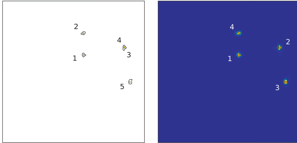
FIG. 4.6. For the potential of Figure 1.1, the correspondence between eigenfunctions and wells of the effective potential does not respect the ordering of the well minima. Moreover, the third and fourth minima effectively define a single well.
