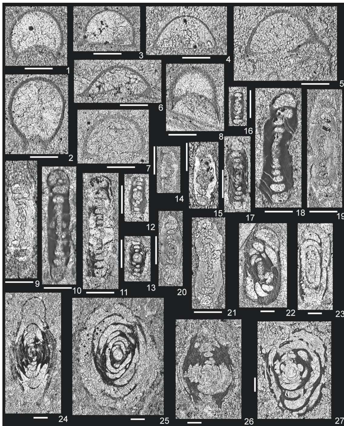
Fig. 5. Foraminifera from the Upper Permian, Changhsingian; “Bituminous limestone” (Bellerophon) Formation; Sitarička Glavica section, Jadar Block, NW Serbia. 1–8 — “ Eotuberitina reitlingerae ” Miklukho-Maklay, axial sections. 1, 3 — sample KM2, thin section 71576; 2, 5, 8 — sample KM4, thin section 71614; 4 — sample KM2, thin section 71611; 6, 7 — sample KM4B, thin section 71876; 9–11 — Hemigordius komiricensis Nestell, Sudar, Jovanović & Kolar-Jurkovšek. 9 — axial section of a completely recrystallized specimen, 10 — close to axial section, 11 — axial section of a partly recrystallized specimen. 9 — sample KM1, thin section 71562; 11 — sample KM4A, thin section 71873; 12–16 — Hemigordius latisspiralis Lin, Li & Sun. 12, 13, 16 — axial sections, 14, 15 — axial sections of completely recrystallized specimens. 12 — sample KM4, thin section 71614; 13 — sample KM4F, thin section 71877; 14 — sample KM11, thin section 71565; 15 — sample KM1, thin section 71562; 16 — sample KM4G, thin section 71832; 17–21 — Hemigordius hungaricus Bérczi-Makk, Csontos & Pelikán. 17, 18 — close to axial sections, 19, 20, 21 — axial sections of completely recrystallized specimens. 17 — sample KM4F, thin section 71880; 18 — sample KM4, thin section 71568; 19, 20 — sample KM10, thin section 71560; 21 — sample KM11, thin section 71565; 22 — Midiella sp., axial section, sample KM4, thin section 71614; 23 — Agathammina cf. A. ovata Wang, close to axial section, sample KM4A, thin section 71833; 24, 25 — Multidiscus vlasticensis Nestell, Sudar, Jovanović & Kolar-Jurkovšek. 24 — axial section, 25 — transverse section; sample KM4E, thin section 71879; 26 — Neodiscus sp. 1, close to axial section, sample KM4B, thin section 71876; 27 — Neodiscus sp. 2, close to axial section, sample KM4B, thin section 71836. Scale bar 100 µm.
