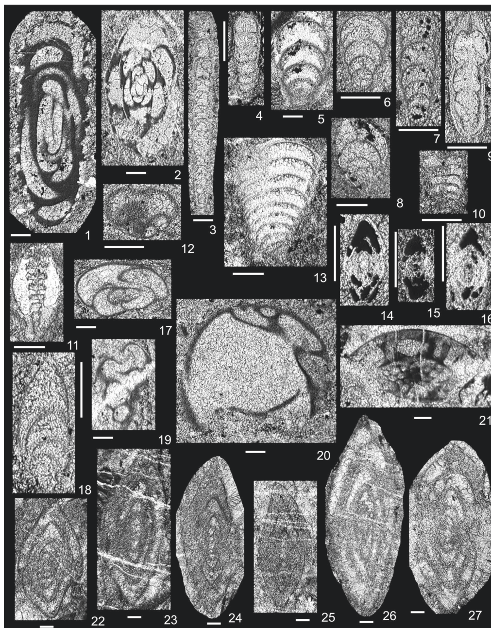
Fig. 6. Foraminifers from the Upper Permian, Changhsingian; “Bituminous limestone” (Bellerophon) Formation; Sitarička Glavica section, Jadar Block, NW Serbia. 1 — Agathammina cf. A. psebaensis Pronina-Nestell, close to axial section, sample KM4, thin section 71614; 2 — Agathammina sp. 1, axial? section, sample KM2, thin section 71611; 3 — Protonodosaria mirabilis caucasica (K. Miklukho-Maklay), close to axial section, sample KM4B, thin section 71876; 4 — Protonodosaria delicata (Wang), close to axial section, sample KM4G, thin section 71832; 5 — Pseudolangella conica (K. Miklukho-Maklay), close to axial section, sample KM4, thin section 71614; 6, 7 — Fronndina cf. F. paraconica (K. Miklukho-Maklay). 6 — axial tangential section, sample KM2, thin section 71613; 7 — lateral section, sample KM4B, thin section 71876; 8 — Fronndina sp. 1, axial tangential section, sample KM9, thin section 71559; 9 — Cryptomorphina limonitica Sellier de Civrieux & Dessauvagie, axial section, sample KM4F, thin section 71880; 10 — Geinitzina cf. G. orientalis K. Miklukho-Maklay, close to axial section, sample KM2, thin section 71576; 11 — Pachyphloia cukurkoyi Sellier de Civrieux & Dessauvagie, axial lateral section, sample KM7, thin section 71573; 12 — Globalbulimina lukachiensis Nestell, Kolar-Jurkovšek, Jurkovšek & Aljinović, tangential section, sample KM4B, thin section, 71836; 13 — Geinitzina cf. G. uralica simplex K. Miklukho-Maklay, axial tangential section, sample KM2, thin section 71613; 14–16 — Robuloides acutus Reichel, axial sections. 14 — sample KM4F, thin section 71877; 15 — sample KM2, thin section 71613; 16 — sample KM4C, thin section 71878; 17 — ?Retroseptellina nitida (Lin, Li & Sun), tangential section, sample KM6, thin section 71561; 18 — Astacolus permicus (K. Miklukho-Maklay), close to axial section, sample KM4B, thin section 71836; 19 — Dagmarita sp., axial tangential section, sample KM4B, thin section 71836; 20 — Paraglobbulimina cf. P. gracilis Zaninetti & Altiner, tangential section, sample KM4, thin section 71614; 21 — ?Palaeofusulina sp., tangential section, sample KM4A, thin section 71873; 22–26 — Nankinella cf. N. chongyangensis Jing, close to axial section, sample KM4, thin section 71568; 23–26 — Nankinella cf. N. acuta Lin, axial sections. 23 — sample KM4, thin section 71568; 24, 25, 26 — sample KM4, thin section 71614; 27 — Staffella cf. S. hupehensis Jing, axial section, sample KM4, thin section 71615. Scale bar 100 \mu m.
