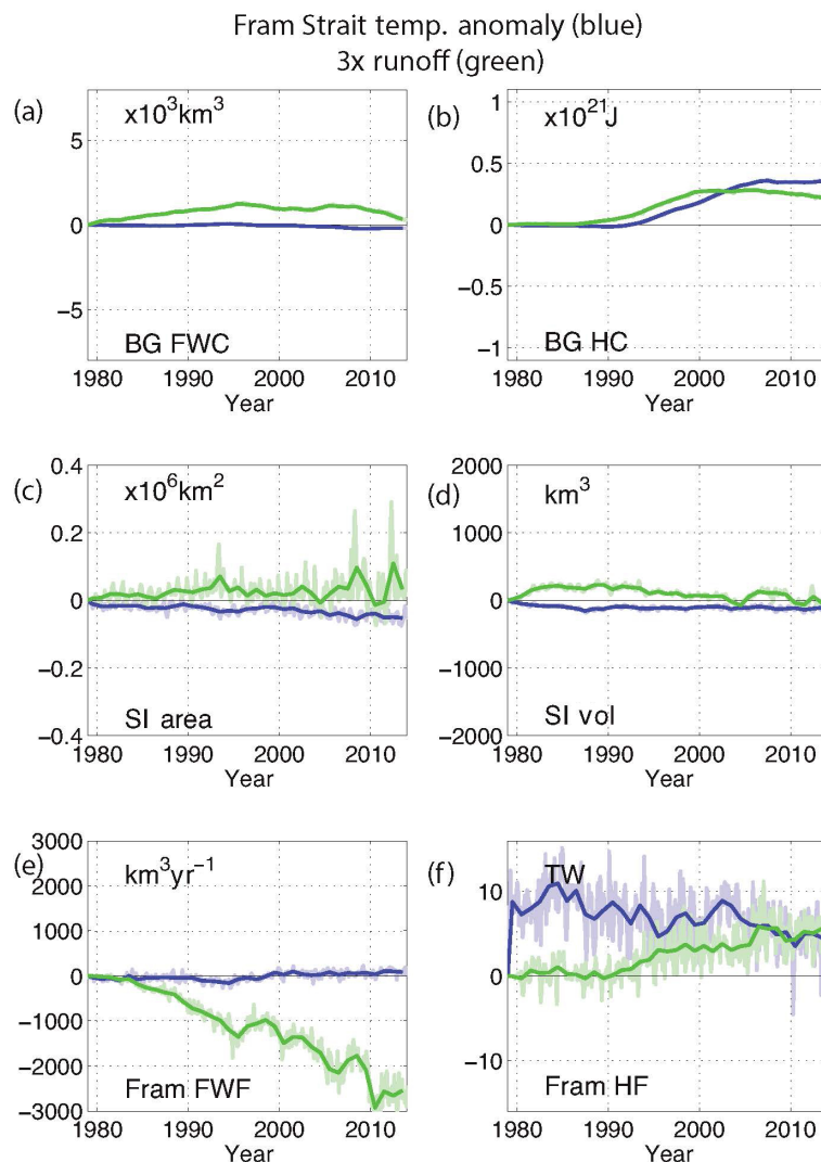
Figure 8. CRFs in response to an impulsive 3 \times Runoff (green lines) and Fram Strait T ( +2C ) anomaly (blue lines): (a) the FWC of the BG (b) HC of the BG (c) SI area (d) SI volume (e) FWF through the Fram Strait, and (f) the HF through the Fram Strait. Note that the units of the y axis appear in the top-left-hand corner of each panel.
