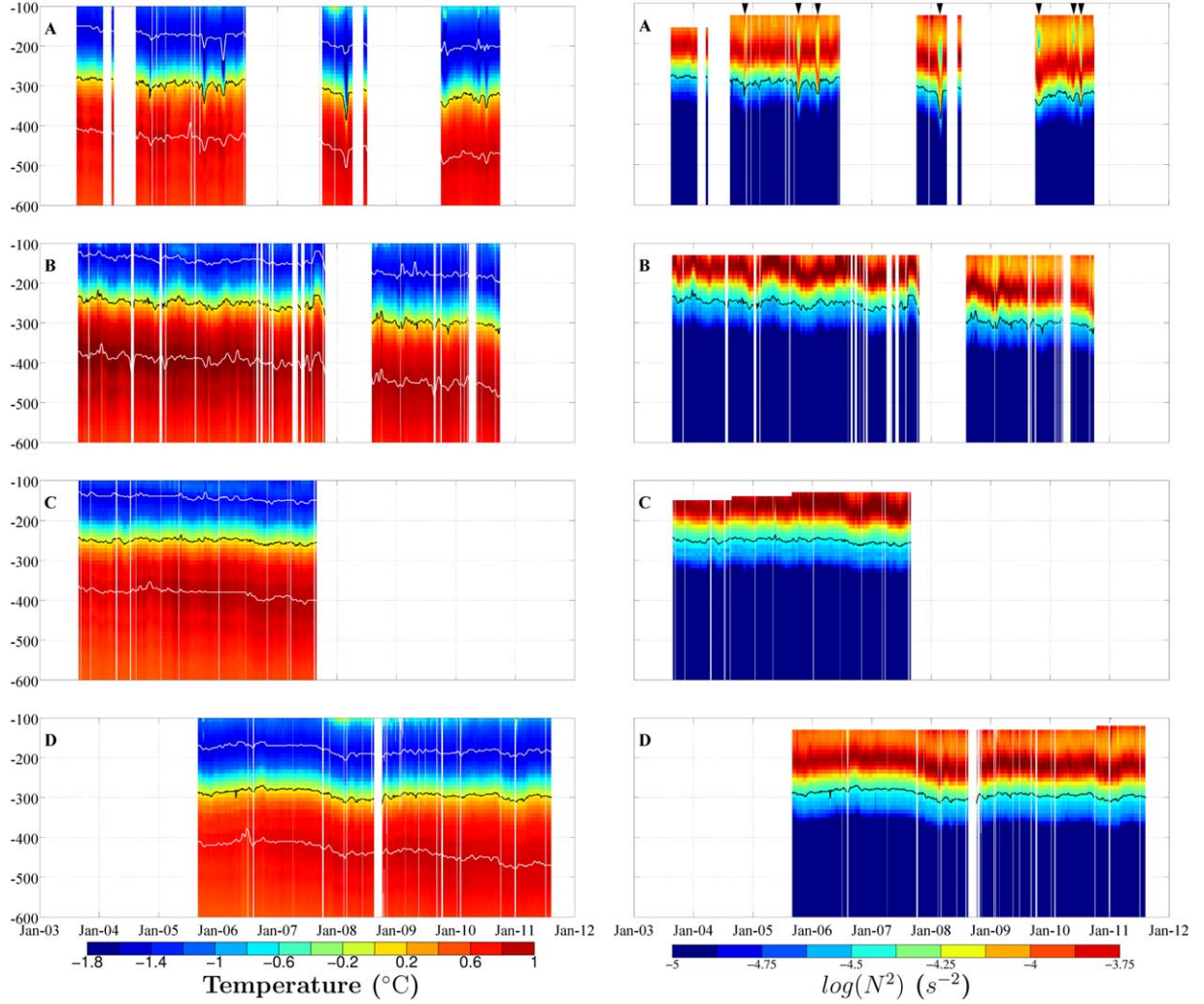
Figure 3. Temperature and buoyancy frequency as a function of time and depth for the moorings A, B, C, and D (from top to bottom). The black line indicates the depth of the 0°C contour for the temperature that represents the limit of the AW temperature. The two white lines indicate the depth of the maximum (lower one) and the minimum (upper one) temperatures. The black arrow on the right top plot indicates the presence of eddies.
