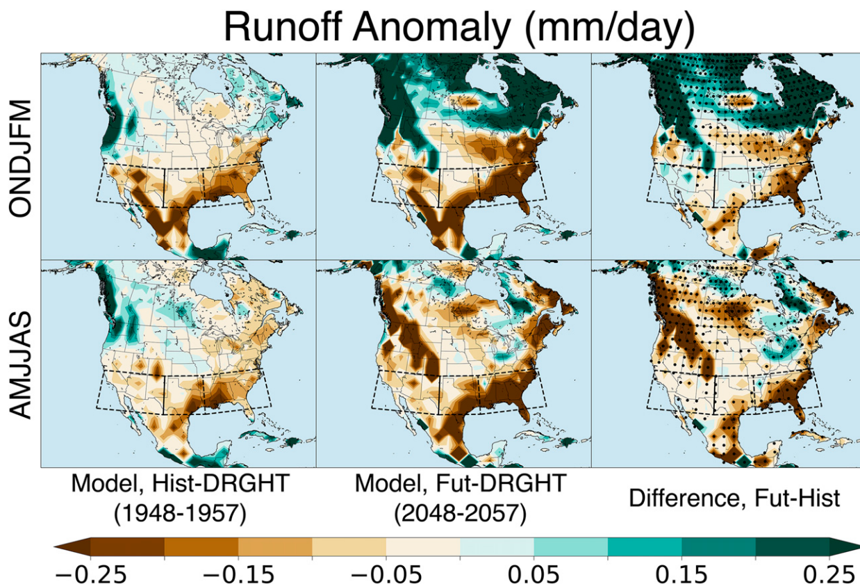
FIG. 8. Ensemble-average (top) cold season (ONDJFM) and (bottom) warm season (AMJJAS) total runoff (combined surface and subsurface) anomalies ( \text{mm day}^{-1} ) during the (left) Hist-DRGHT (1948–57) and (center) Fut-DRGHT (2048–57) intervals, relative to the 1891–1920 baseline average. (right) Differences between the two drought periods (Fut-DRGHT minus Hist-DRGHT). Areas where these runoff anomalies are significantly different between the two drought periods (based on a two-sided Kolmogorov–Smirnov test, p \leq 0.05 ) are indicated by the black stippling.
