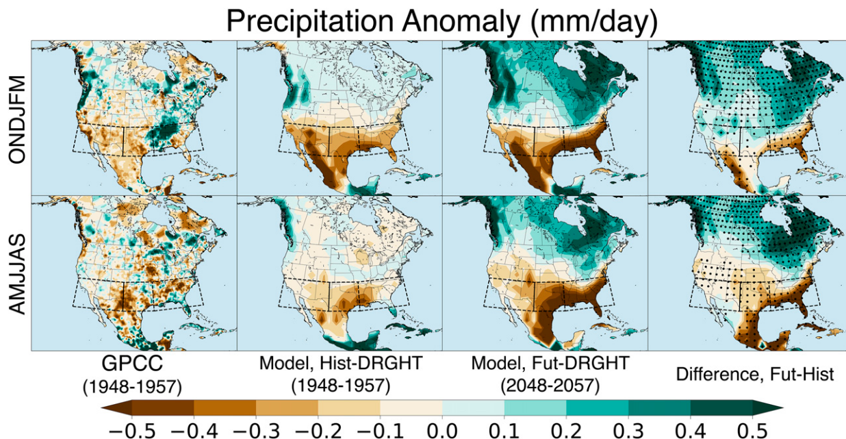
FIG. 5. Observed (GPCC) and modeled (ensemble average) (top) cold season (ONDJFM) and (bottom) warm season (AMJJAS) precipitation anomalies ( \text{mm day}^{-1} ) during the Hist-DRGHT (1948–57) and Fut-DRGHT (2048–57) intervals, relative to the 1891–1920 baseline average. Simulated Hist-DRGHT precipitation anomalies are broadly similar to observations (GPCC), with deficits across the Southwest, Mexico, southern plains, and Southeast United States, especially during the cold season. (right) Differences between the two drought periods (Fut-DRGHT minus Hist-DRGHT), showing amplified drying in Fut-DRGHT over the Southeast in both seasons and the southern plains and Southwest in the warm season, along with reduced deficits over much of the Southwest in the cold season. Areas where precipitation anomalies are significantly different between the two drought periods (based on a two-sided Kolmogorov–Smirnov test, p \leq 0.05 ) are indicated by the black stippling.
