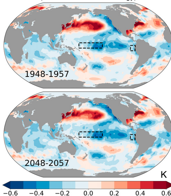
FIG. 1. (top) Linear trend ( \text{K yr}^{-1} ) in December–February (DJF) SSTs from 2015 to 2100. (bottom) DJF SST anomalies during Hist-DRGHT (1948–57, calculated relative to 1935–70) and Fut-DRGHT (2048–57, calculated relative to 2035–70). Dashed areas indicate the Niño-4 ( 5^{\circ}\text{N} – 5^{\circ}\text{S} , 160^{\circ}\text{E} – 150^{\circ}\text{W} ) and Niño-1+2 ( 0^{\circ} – 10^{\circ}\text{S} , 90^{\circ} – 80^{\circ}\text{W} ) regions.
