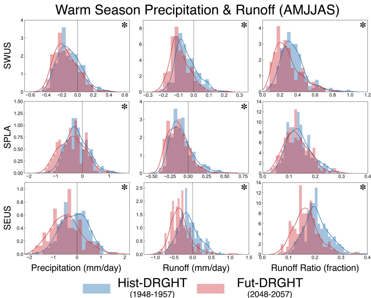
FIG. 11. Normalized histograms (bars) and kernel density plots (lines) for warm season (AMJJAS) average (left) precipitation anomalies, (center) runoff anomalies, and (right) runoff ratios, averaged over (top) SWUS, (middle) SPLA, and (bottom) SEUS. Distributions include all years from the Fut-DRGHT and Hist-DRGHT periods (10 in each ensemble member) from all 20 ensemble members ( n = 200 ). Black asterisks indicate variables with significant ( p \leq 0.05 ) differences between Fut-DRGHT and Hist-DRGHT, based on a two-sided Kolmogorov–Smirnov test.
