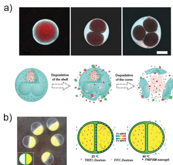
Fig. 12 Multicompartment microparticles for coencapsulation of multi-drugs. (a) CLSM images of DOX (red) and CPT (blue) loaded microparticles with single or multiple cores, and illustration of sequenced fracture of the shell and the core to release the drugs. 147 Reprinted with permission from ref. 147. Copyright 2017, Science China Press. (b) Optical micrograph of microcapsules with dual compartments and heterogeneous shell, and illustration of microcapsules exhibiting both temperature triggered release and sustained release. 148 Reprinted with permission from ref. 148. Copyright 2016, American Chemical Society.
