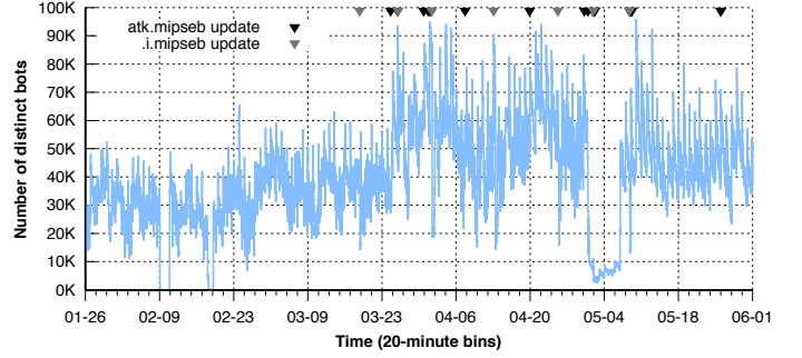
Fig. 2: Number of unique Hajime bots. (Active scans.)
