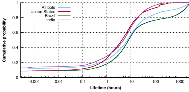
Fig. 6: CDF of a Hajime bot’s lifetime. We show the overall lifetime of all bots, and break it down into three of the top countries. (Active scans, 01/26/2018 – 05/31/2018.)
