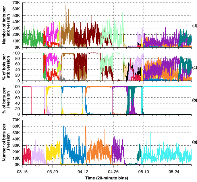
Fig. 10: Propagation of Hajime updates for mipseb architecture payloads. All four plots use the same X-axis time scale. (Active scans.)
