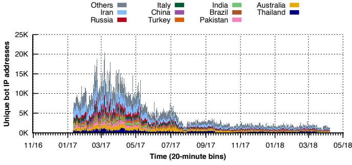
Fig. 13: Unique bot IP addresses for the top-10 countries with the most overall unique bot IP addresses (DNS backscatter, 12/27/2016 – 04/08/2018.)
