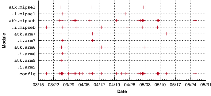
Fig. 1: Hajime updates. There were 50 config updates during the period 03/18/2018 – 05/31/2018.
