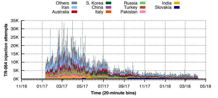
Fig. 14: Injection attempts for the top-10 countries with the most overall Hajime injection attempts (DNS backscatter, 12/27/2016 – 04/08/2018.)
