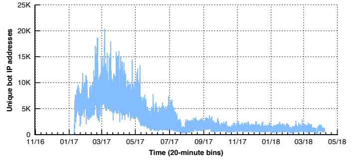
Fig. 12: Unique Hajime bot IP addresses. (DNS backscatter, 12/27/2016 – 04/08/2018.)
