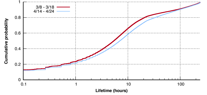
Fig. 5: CDF of a Hajime bot’s lifetime during two “stable” periods with no i updates. (Active scans.)
