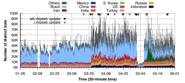
Fig. 7: Number of unique Hajime bots for the 10 most prevalent countries. (Active scans.)
