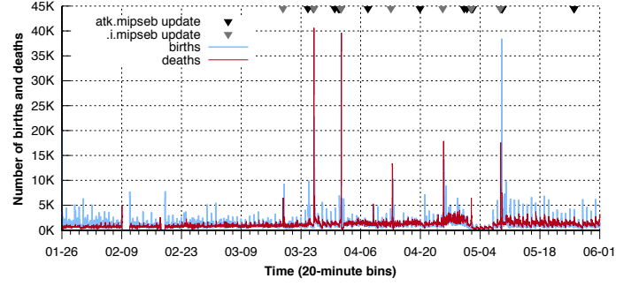
Fig. 4: Bot churn in Hajime. “Births” denote the first time we saw a given key, “deaths” denote the last time. (Active scans.)
