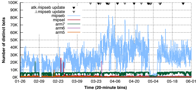
Fig. 8: Number of Hajime bots, broken down by architecture. (Active scans.)
