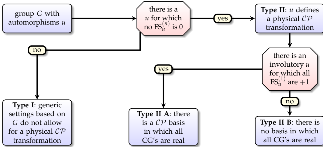
FIGURE 3: The regular and extended twisted Frobenius-Schur indicators FS_u and FS_u^{(n)} allow us to distinguish between the three types of groups. Here, n is n = \text{ord}(u)/2 for even and n = \text{ord}(u) for odd \text{ord}(u) . From [1].
