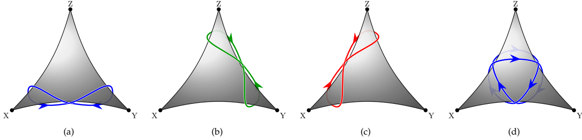
FIGURE 4: Winding strings. Linear combinations of 4a–4c give rise to three \Delta(54) doublet representations while 4d leads to the fourth and last one.
