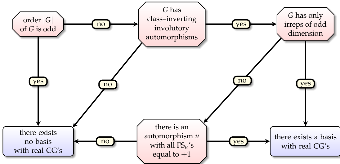
FIGURE 2: Sequence of steps to determine whether or not a group admits a basis in which all CG's are real. From [1].
