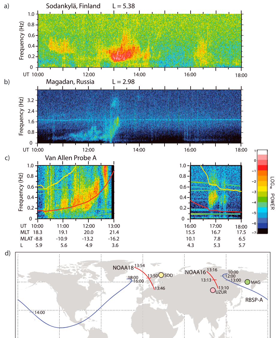
Figure 7. Composite figure showing spectrograms of the By (eastward) components of magnetic field data from Sodankylä, Finland (a), Magadan, Russia (b), and Van Allen Probe A (c) from 10:00 to 18:00 UT 24 September 2013 and a map (d) showing the Northern Hemisphere magnetic footprints of Van Allen Probe A from 10:00 to 18:00 UT, of NOAA 16 from 13:12 to 13:14 UT, and of NOAA 18 from 13:45 to 13:55 UT, respectively, on 24 September 2013. The locations of Magadan, Uzur, and Sodankylä are indicated by green, pink, and yellow circles, respectively. UT = universal time; MLT = magnetic local time; MLAT = magnetic latitude; NOAA = National Oceanic and Atmospheric Administration; RBSP-A = Radiation Belt Storm Probe-A (Van Allen Probe A).
