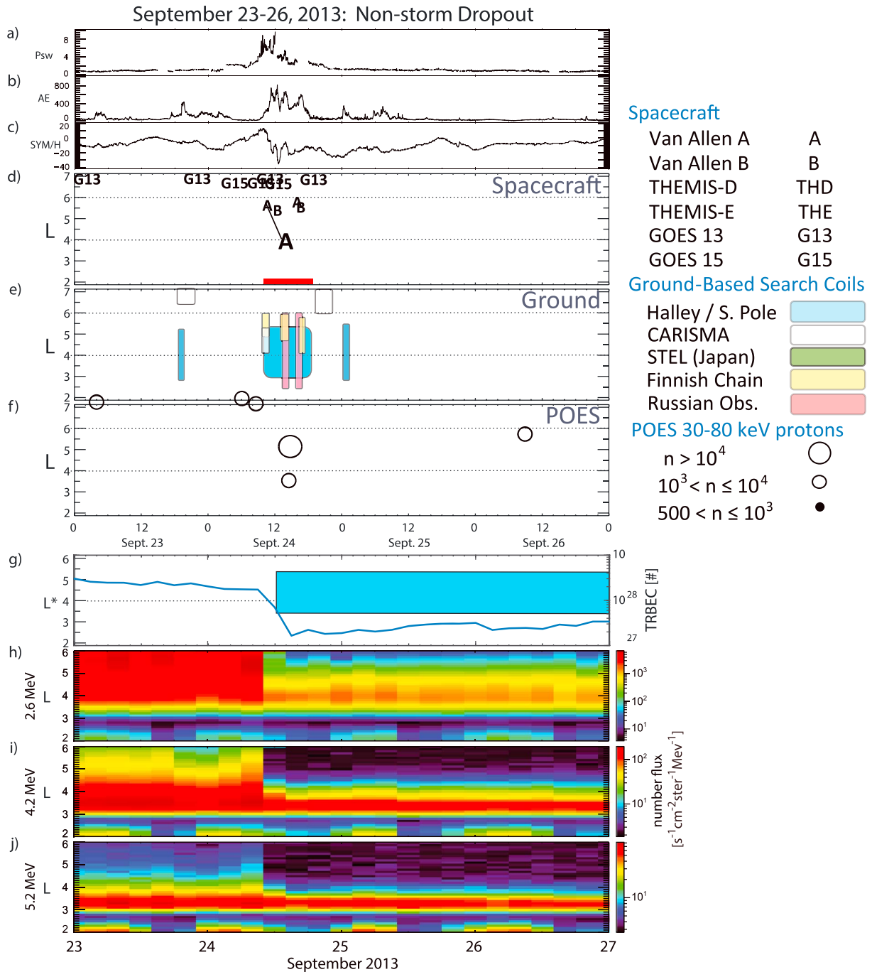
Figure 5. Nonstormtime dropout interval from 23 September through 26 September 2013. (a), (b), and (c) show the solar wind dynamic pressure (Psw), the 1-min AE index, and the 1-min SYM/H index, respectively. (d), (e), and (f) summarize EMIC wave activity as a function of L and universal time observed in situ by spacecraft magnetometers, by ground-based induction magnetometers, and by POES proton detectors, respectively, according to the legends on the right. The red bar at the bottom of (d) indicates an interval of ground-based observations of intense EMIC waves. (g) shows the total radiation belt electron content (TRBEC, scale on the right), and the blue box indicates the L^* and universal time ranges in which EMIC wave-induced depletions of ultrarelativistic electrons were observed. (h), (i), and (j) show spin-averaged differential fluxes of relativistic and ultrarelativistic electrons measured by the Relativistic Electron-Proton Telescope instrument on Van Allen Probes A and B in three energy channels: 2.6, 4.2, and 5.2 MeV. EMIC = electromagnetic ion cyclotron; POES = Polar Operational Environmental Satellite; THEMIS = Time History of Events and Macroscale Interactions during Substorms; GOES = Geostationary Operational Environmental Satellite; CARISMA = Canadian Array for Realtime Investigations of Magnetic Activity.
