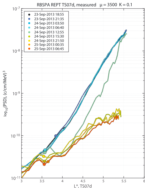
Figure 8. Phase space densities (PSDs), in units of (\text{c}/\text{cm}/\text{MeV})^3 , of ultrarelativistic electrons with \mu = 3,500 \text{ MeV}/\text{G} and K = 0.1 \text{ G}^{0.5} R_E observed by Van Allen Probe A during its passes from 18:55 universal time 23 September through 06:45 universal time 25 September 2013. Each filled circle corresponds to the closest point in time when a valid PSD observation was available near a given L^* value of interest, in this case L^* = 3.6 . These times are given in the legend of the figure, next to the corresponding color. Values of L^* were calculated based on the TS07d magnetic field model. RBSPA = Radiation Belt Storm Probe A; REPT = Relativistic Electron-Proton Telescope.
