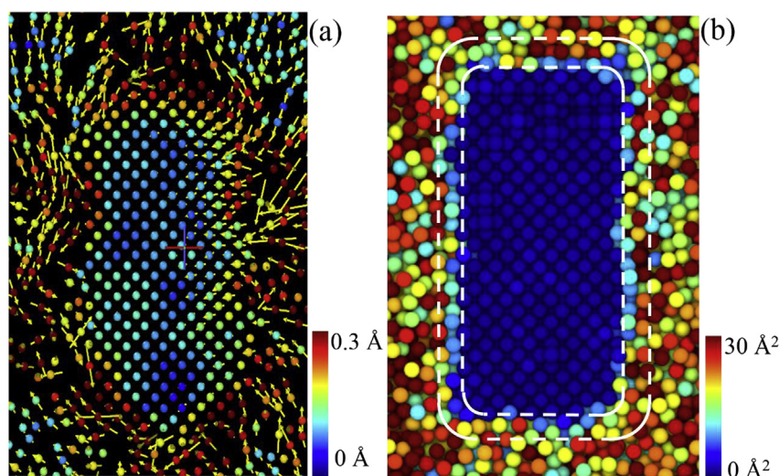
Fig. 4. (a) The atomic displacement (yellow arrows) and local shear strain (atomic color) diagram of the portion of the S1 nanocomposite at the strain of 4%; (b) The common neighborhood parameter of the portion of the S1 nanocomposite at the strain of 4%, the interface is shown in a white rectangle. (For interpretation of the references to color in this figure legend, the reader is referred to the Web version of this article.)
