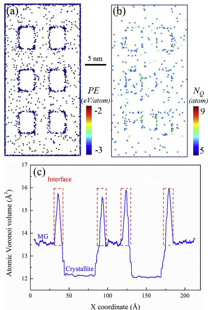
Fig. 3. (a) Potential energy, and only atoms with potential energy larger than -3 eV/atom are displayed. (b) Defects in the interfaces, characterized by QNA, and only atoms with the number of QNA ( N_Q ) larger than 5 atoms are shown at the initial configuration prior to deformation in the S2 nanocomposite. (c) Distribution of atomic Voronoi volume along the X coordinate (in the direction perpendicular to the loading direction).
