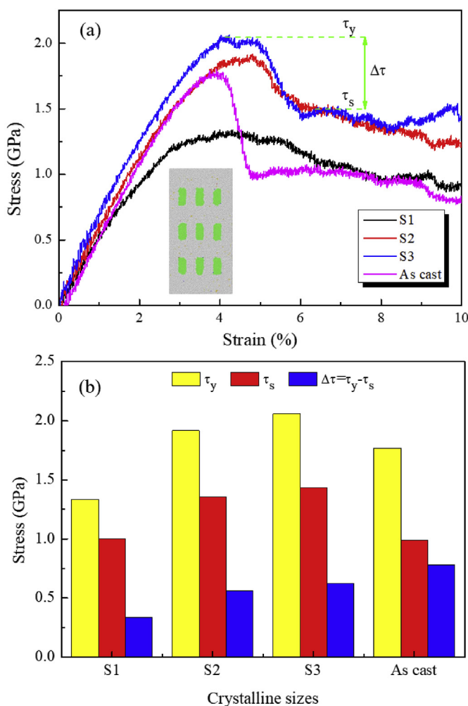
Fig. 1. (a) Stress-strain curves of nanocomposites with different crystalline sizes: S1, S2, S3 and as cast. The insert shows the schematic of the S1 nanocomposite. Green represents crystallites, while gray represents MGs. (b) \tau_y is to the global yield strength and \tau_s is regarded as the flow strength. \Delta\tau = \tau_y - \tau_s corresponds to a change in stress response. (For interpretation of the references to color in this figure legend, the reader is referred to the Web version of this article.)
