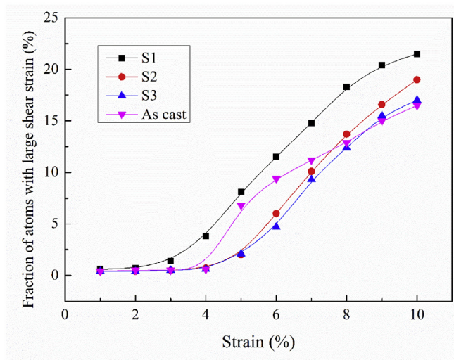
Fig. 8. The proportions of atoms with \eta_{\text{Mises}} greater than the threshold value of 0.2 for the nanocomposites at different strains.
