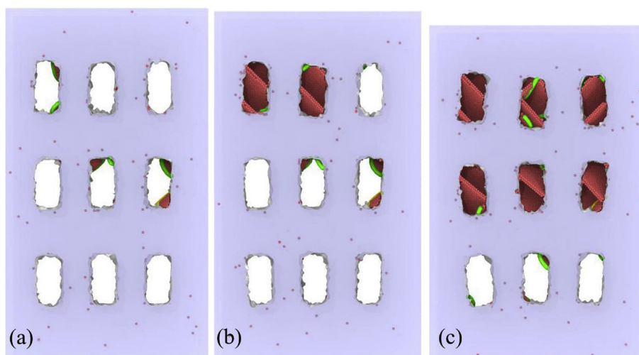
Fig. 5. 1/6\langle 112 \rangle (Shockley) partial dislocation (green lines) and stacking fault (red atoms) of the S1 nanocomposite at strains of (a) 4%, (b) 5% and (c) 10%. For simplicity, all atoms belonging to the FCC structure are deleted. (For interpretation of the references to color in this figure legend, the reader is referred to the Web version of this article.)
