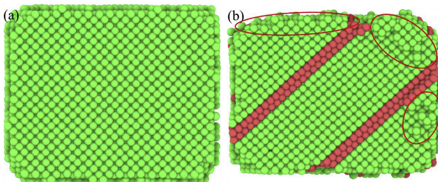
Fig. 6. Atomic structure of the crystallites at strains of (a) 0% and (b) 10%. Green represents FCC, while red represents stacking faults formed via atomic shuffling. The red ovals denote dissolution processes of the FCC crystallites. (For interpretation of the references to color in this figure legend, the reader is referred to the Web version of this article.)
