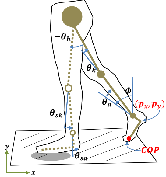
Fig. 1. Kinematic model of the biped. COP denotes the Center of Pressure. The solid links denote the stance leg, the dashed links denote the swing leg.
