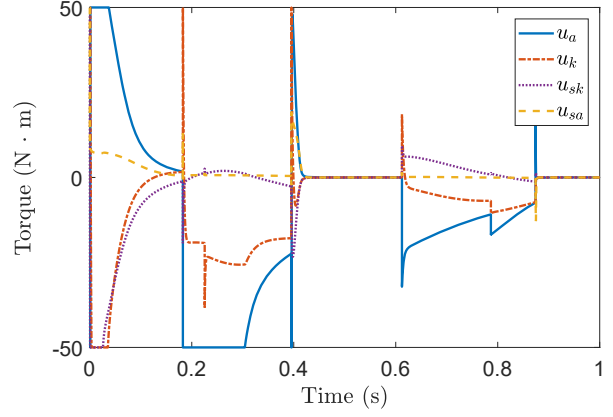
Fig. 4. Torque over time for the centralized controller U for the first three steps
