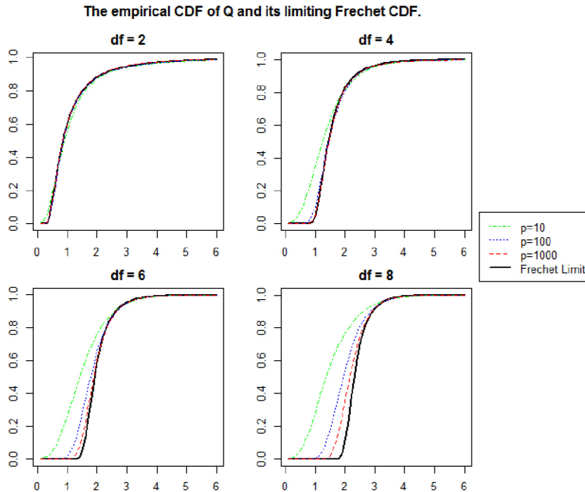
Fig. 2. Finite sample empirical distribution of the maxima Q and its corresponding Fréchet limit, with different combinations of p and degrees of freedom ( df ) of the t -distribution in the factor model.
