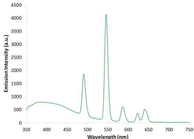
Fig. 2 Room temperature emission spectrum of the \text{Tb}^{3+} complex of 3 in methanol ( [\text{Tb-3}] = 2.0 \times 10^{-3} \text{ M} , \lambda_{\text{ex}} = 320 \text{ nm} ).
