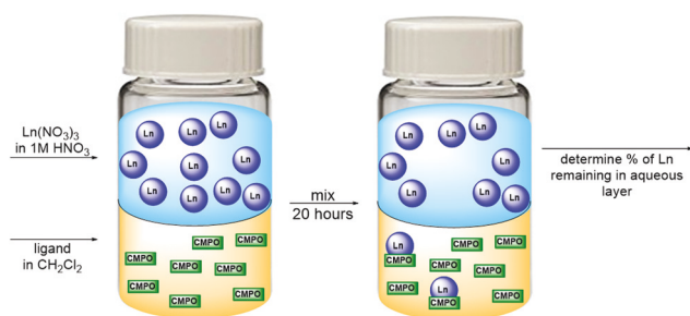
Fig. 3 Schematic illustration of liquid–liquid extraction protocol used in this study. Following mixing, the aqueous phase was analyzed by either the traditional Arsenazo III absorption assay, or via ICP-AES to determine Ln ion concentration.
