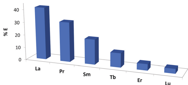
Fig. 4 Consistent trend toward decreasing percent extraction for TREN-CMPO-Ph ( 4 ) through the Ln 3+ series achieved utilizing a 100 : 1 ligand to metal ratio (values with standard deviations given in Table S1†). Extraction experiments were performed with 4 dissolved in CH 2 Cl 2 (10 −2 M) mixed with equal volumes of each individual Ln nitrate solution ([Ln 3+ ] = 10 −4 M in 1 M HNO 3 ), stirring for 20 h at room temperature.
