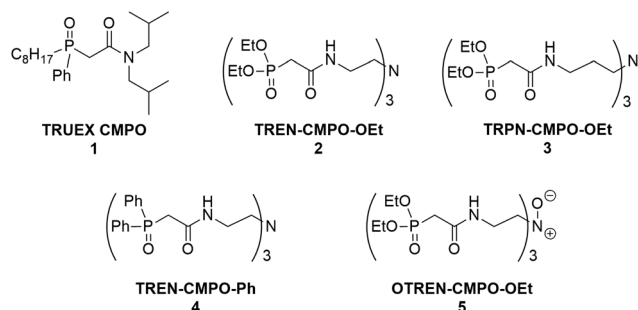
Fig. 1 Monopodal CMPO ligand 1 used in the TRUEX process for nuclear waste remediation and the four tripodal CMPO ligands 2–5 studied herein.
