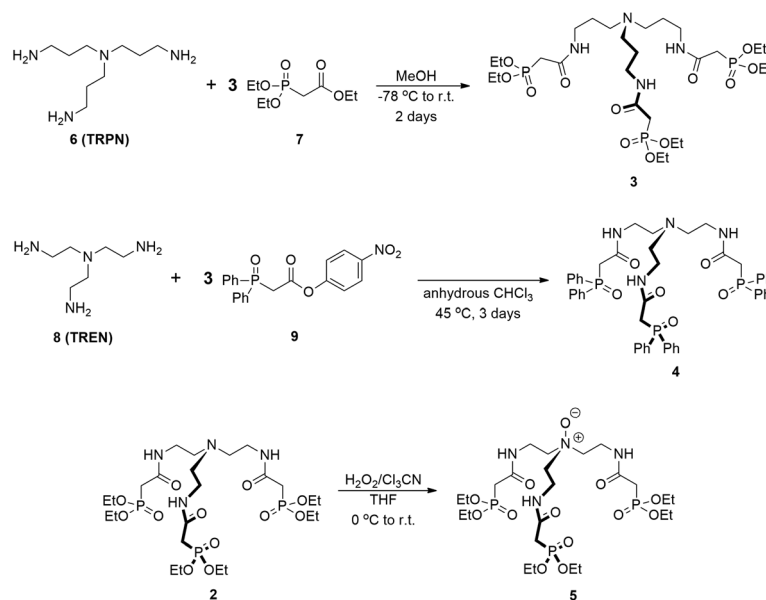
Scheme 1 Synthetic pathways to ligands 3–5.
