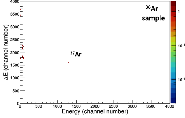
FIG. 10. Same as Fig. 7 for a non irradiated ^{36}\text{Ar} (blank). One ^{37}\text{Ar} count detected for this sample over 6.5 hours, likely due to a memory effect in the ion source, corresponds to a concentration ^{37}\text{Ar}/^{36}\text{Ar}=9 \times 10^{-16} .
