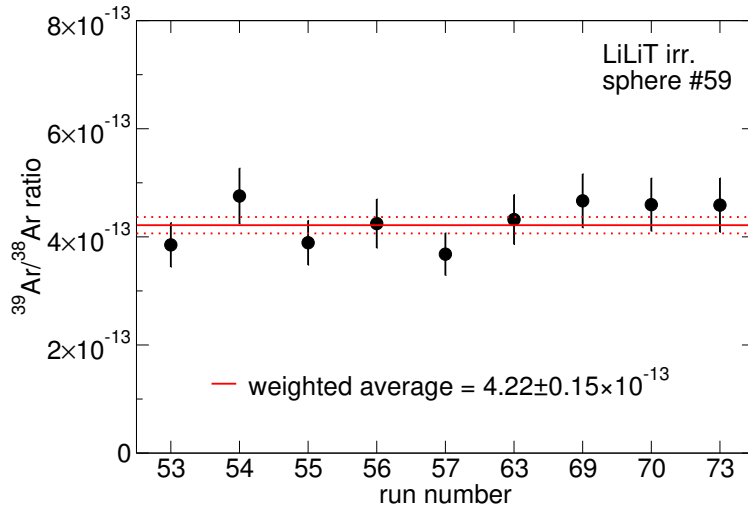
FIG. 16. Repeated measurements of the ^{39}\text{Ar}/^{38}\text{Ar} ratio for the LiLiT irradiated sphere (#59). See Table VIII for numerical results.
