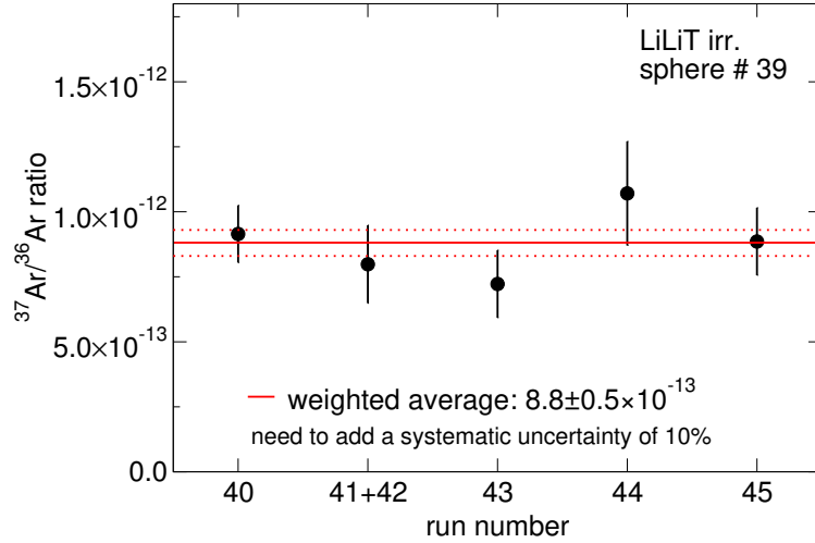
FIG. 12. Repeated measurements of the ^{37}\text{Ar}/^{36}\text{Ar} ratio for the LiLiT irradiated sphere (#39). See Table IV for numerical results.
