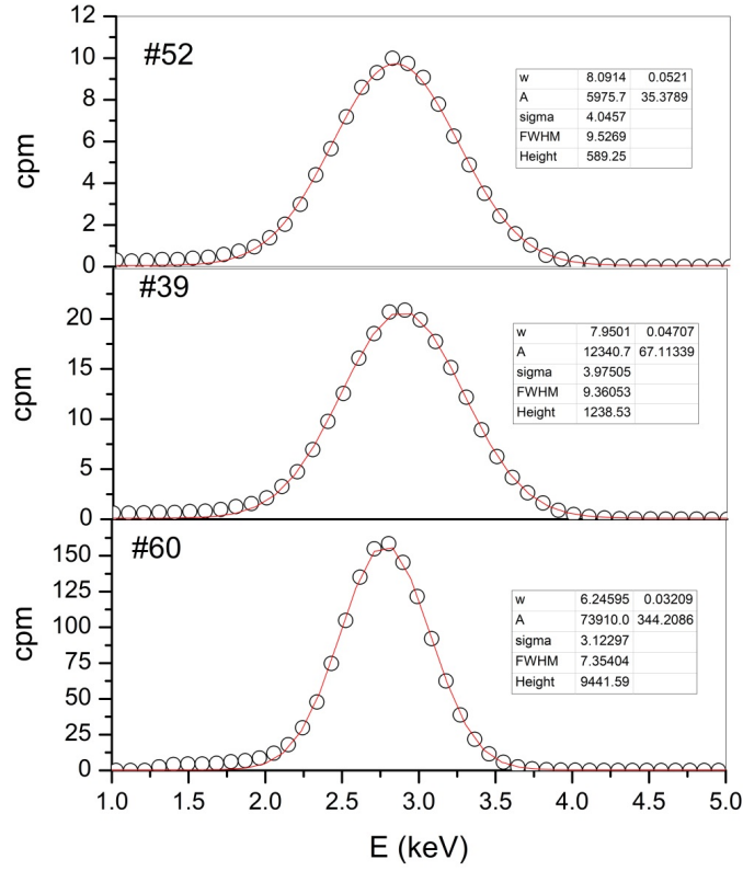
FIG. 14. Energy spectra (in counts per minute) and gauss fit of ^{37}\text{Ar} measurements by low-level counting (LLC). The peak energy correspond to the 2.82 keV K-capture decay energy of ^{37}\text{Ar} .
