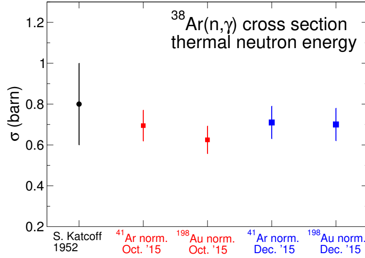
FIG. 19. Comparison of the measured ^{38}\text{Ar} thermal cross section using external ^{198}\text{Au} and internal ^{41}\text{Ar} neutron monitoring.
