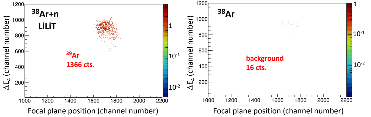
FIG. 11. Two-dimensional spectra of \Delta E_4 vs. focal plane position gated on the ^{39}\text{Ar} region-of-interest in the time-of-flight, \Delta E_2 and \Delta E_3 detector parameters.
