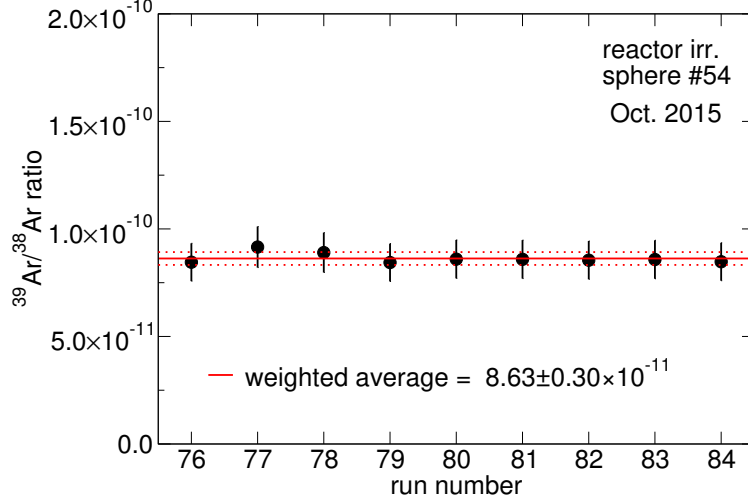
FIG. 17. Same as Fig. 16 for the reactor irradiated sphere (#54). See Table IX for numerical results.
