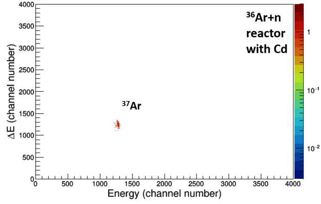
FIG. 8. Same as Fig. 7 for the reactor irradiated sphere with Cd #52a.
