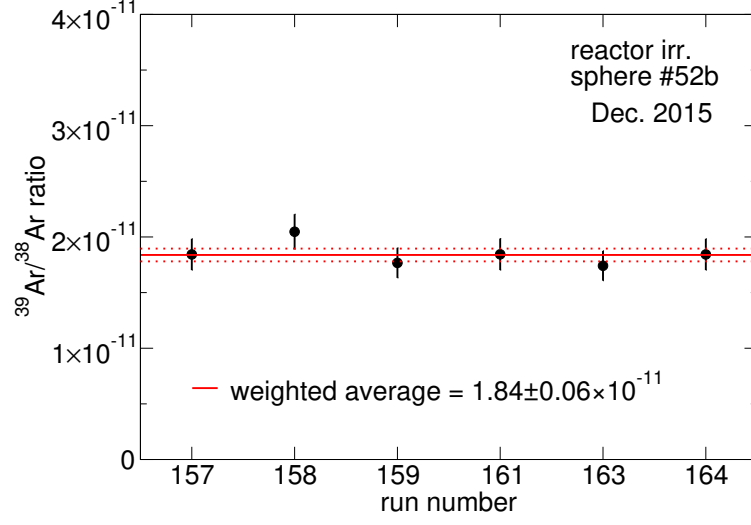
FIG. 18. Same as Fig. 16 for the reactor irradiated sphere (#52b). See Table X for numerical results.
