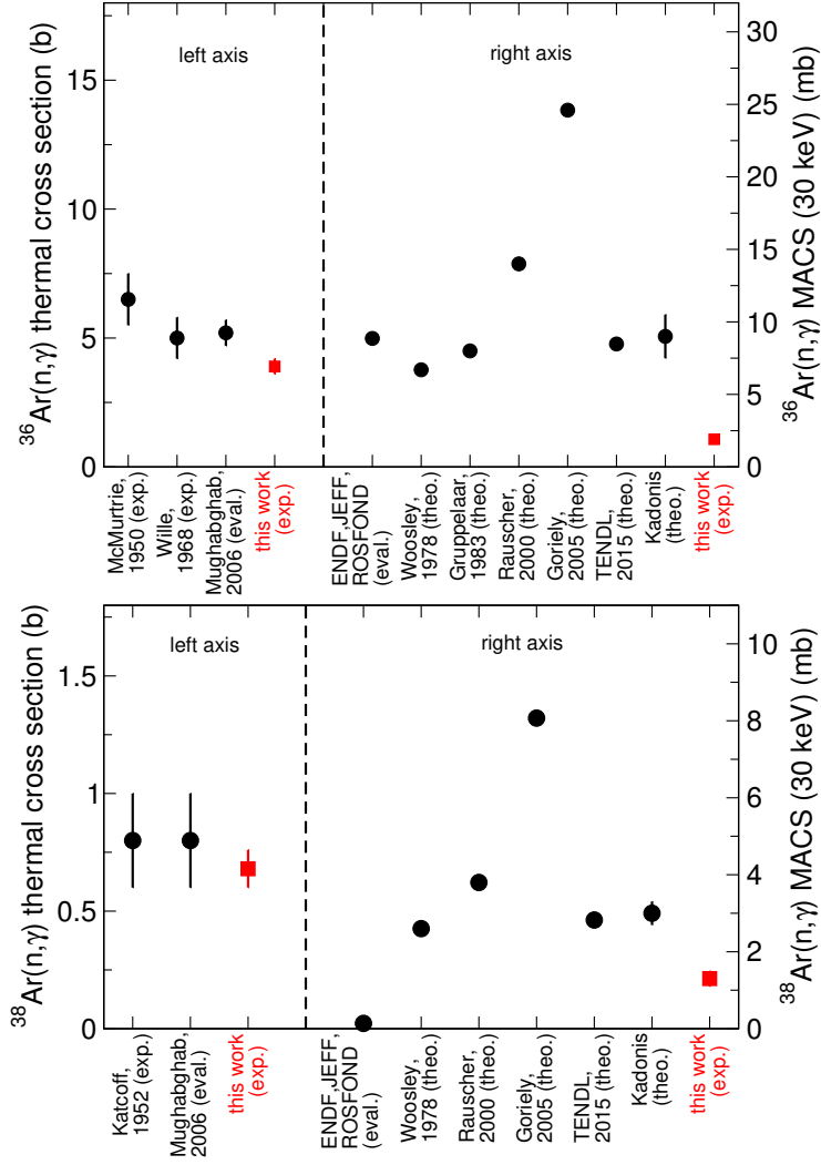
FIG. 21. Comparison of the ^{36}\text{Ar} (top) and ^{38}\text{Ar} (bottom) thermal and Maxwellian Average (30 keV) cross sections measured in this work (red squares) to measured (thermal) and theoretical data (black circles). Numerical values are listed in Table II (main paper).
