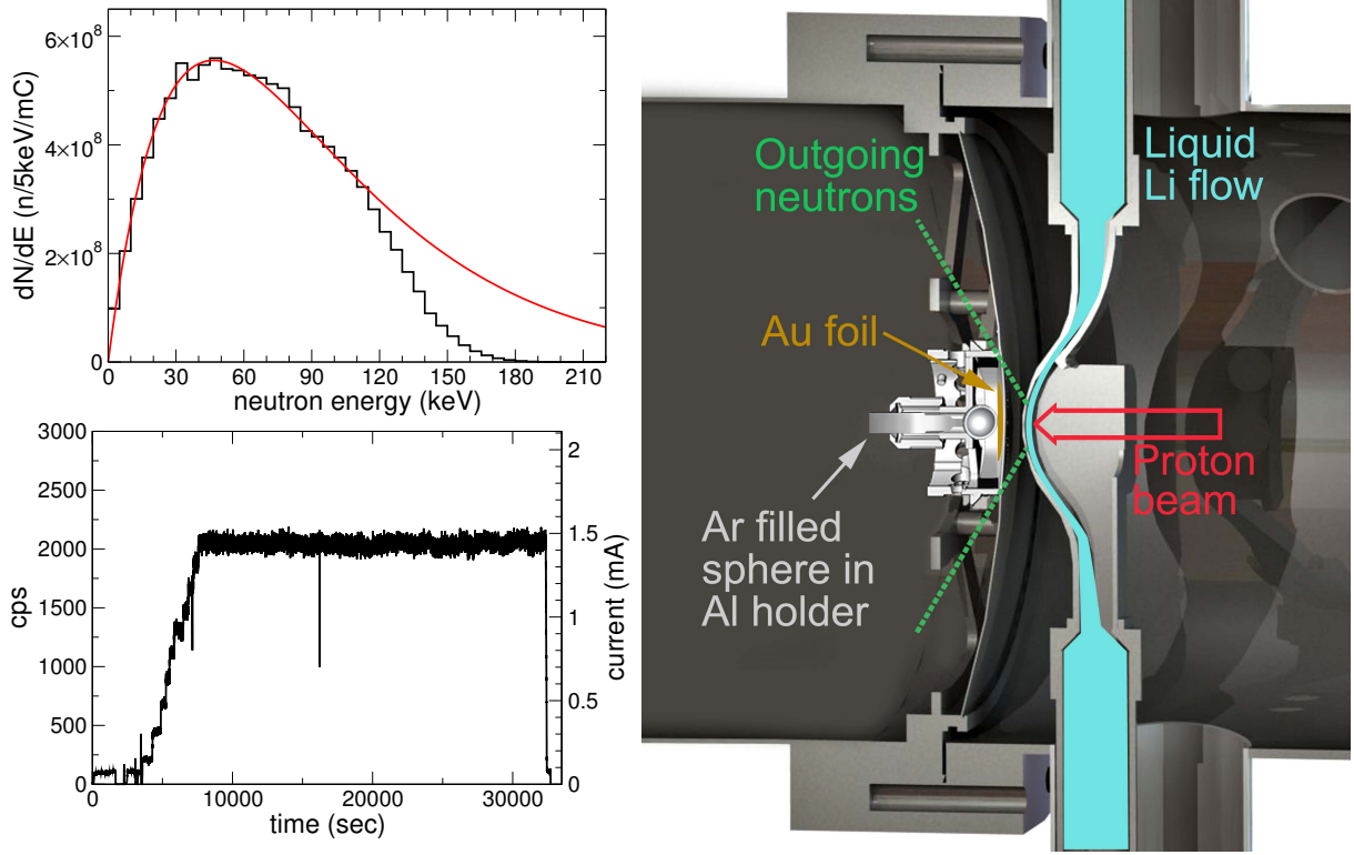
FIG. 1. (Color online) (right) Diagram of the Liquid-Lithium Target (LiLiT) and activation target assembly. The ( \sim 1.5 mA, \sim 9 mm full width) proton beam (open red arrow) impinges on the free-surface lithium film (cyan) (see [19] for details). The Ar-filled sphere and Au foil are positioned in the outgoing neutron cone (green dotted lines) in a vacuum chamber separated from the LiLiT chamber. (top left) Simulated neutron spectrum incident on the ^{36}\text{Ar} sample (black) and a fit in the range E_n \sim 0 - 110 keV with a Maxwell-Boltzmann flux (red) at kT \sim 47 keV. (bottom left) Count rate (left y-axis) of fission chamber (see text) and calibration to proton current (right y-axis) during the ^{36}\text{Ar} run.
