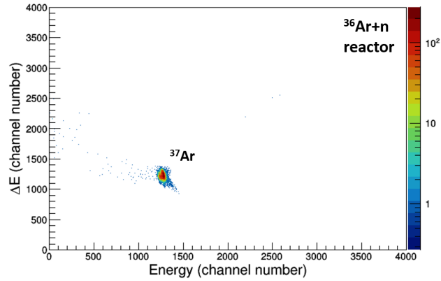
FIG. 9. Same as Fig. 7 for the reactor irradiated sphere (without Cd) #60.
