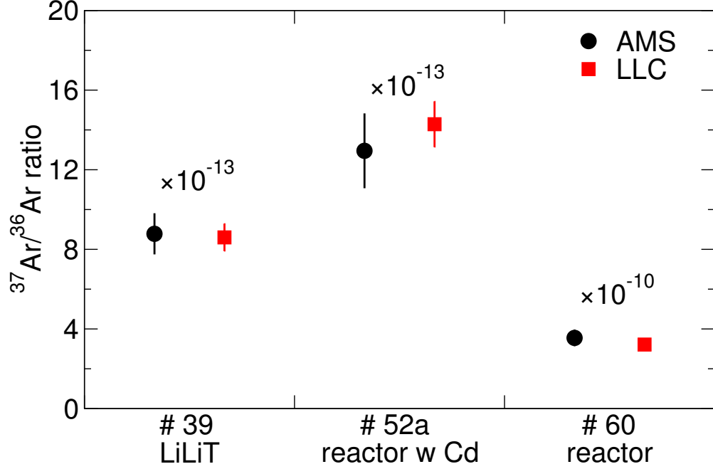
FIG. 2. (Color online) Comparison of the ^{37}\text{Ar}/^{36}\text{Ar} ratio (at the end of irradiation) measured by AMS (black) and LLC (red).
