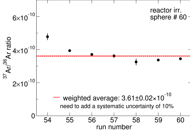
FIG. 13. Same as Fig. 12 for the sphere irradiated at the reactor (#60). See Table VI for numerical results.
