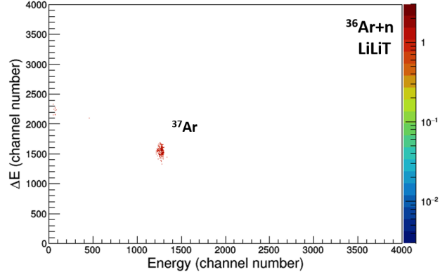
FIG. 7. Identification spectra of the ^{37}\text{Ar} counts with the \Delta E -E telescope of Si detectors for the LiLiT irradiated sphere #39.
