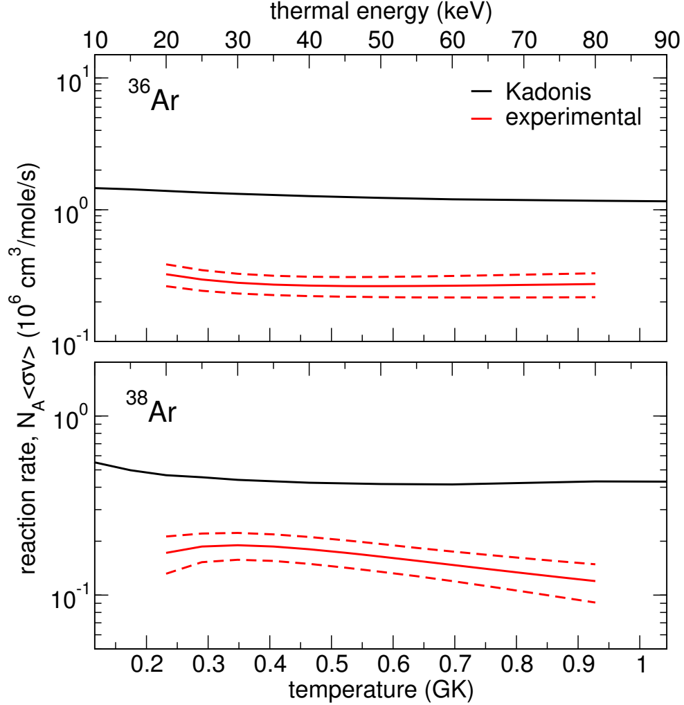
FIG. 4. (Color online) Comparison of the ^{36}\text{Ar} (top) and ^{38}\text{Ar} (bottom) (n, \gamma) reaction rates ( N_A \langle \sigma v \rangle ) extracted from this work (red) to the Kadonis [49] recommended values (black). The dashed curves encompass the estimated 1\sigma uncertainty.
