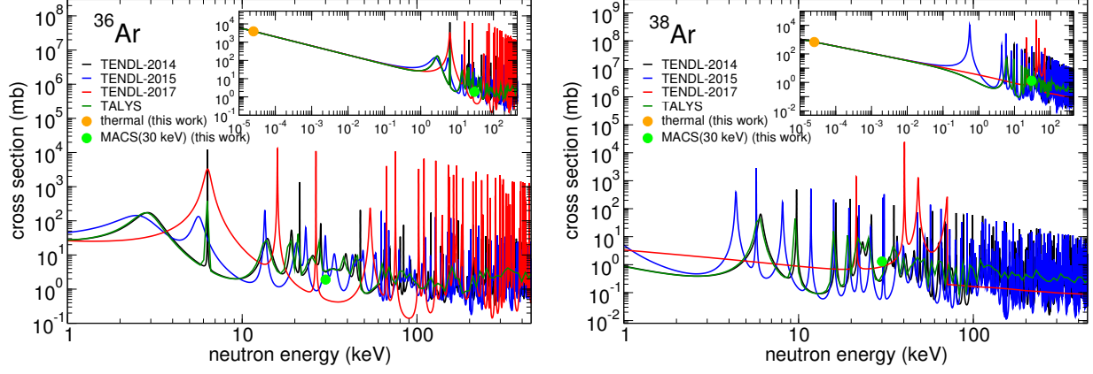
FIG. 20. Excitation functions of the ^{36,38}\text{Ar}(n, \gamma) reaction calculated with the Hauser-Feshbach codes indicated. The experimental values of the thermal cross section and of the MACS(30 keV) determined in this work are shown. The excitation functions are matched to the thermal cross sections measured in this work.
