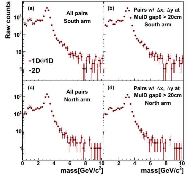
FIG. 35. The mass spectra of MuDLL1-1D triggered data for the (a,b) south arm and (c,d) the north arm are shown separately. Open circles are pairs in which both associated tracks satisfy the MuDLL1-1D condition, while closed circles are pairs in which the associated tracks satisfy the MuDLL1-2D condition. Panels (a,c) show all pairs, while the panels (b,d) show only pairs with a spatial separation exceeding 20 cm at MuID gap 0.
