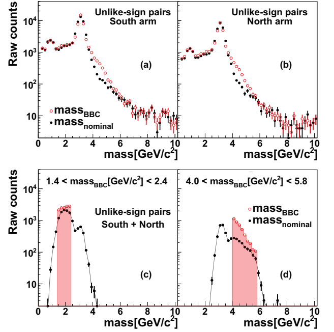
FIG. 4. The mass spectra from the (a) south and (b) north arms, where the mass is calculated with different constraints to the vertex position: (i) a common vertex within \pm 40 cm around the nominal event vertex ( mass_{nominal} , closed circles), and (ii) the vertex measured by the BBC ( mass_{BBC} , open circles). mass_{BBC} and mass_{nominal} distributions are compared with pairs selected with mass_{BBC} (c) between 1.4 and 2.4 GeV/c^2 , and (d) between 4.0 and 5.8 GeV/c^2 .
