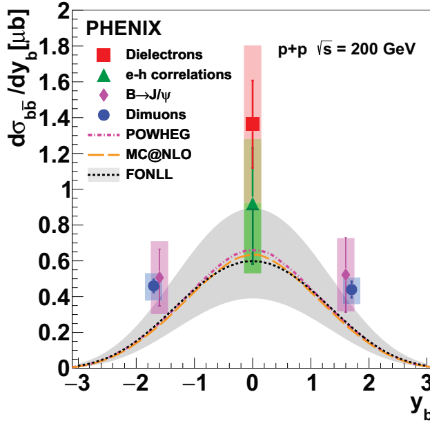
FIG. 27. Rapidity density d\sigma_{b\bar{b}}/dy_b in p+p collisions at \sqrt{s} = 200 \text{ GeV} measured in PHENIX via various channels compared to theoretical calculations. Here y_b is the rapidity of a b quark.
