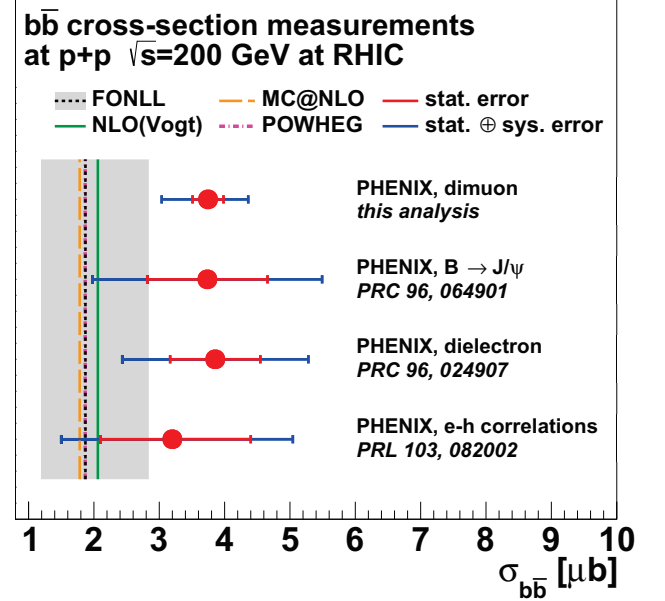
FIG. 28. Bottom cross section \sigma_{b\bar{b}} in p+p collisions at \sqrt{s} = 200 \text{ GeV} measured at RHIC via various channels compared to NLL and NLO calculations. The gray band represents the systematic uncertainty in the FONLL calculation.
