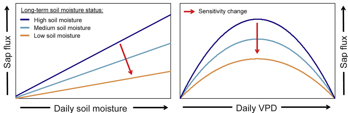
Fig. 1. Hypothetical relationships between sap flux and daily soil moisture or vapor pressure deficit (VPD) variation under different long-term soil moisture conditions (high, medium and low soil moisture). The red arrow indicates changes in sap flux sensitivity to soil moisture and VPD resulting from physiological and possible structural adjustments to soil moisture change (e.g. hydraulic resistance, stomatal density, synthesis of chemicals inducing stomatal closure, rooting depth). Because of adjustments to reduced soil moisture, trees would experience a decreased sensitivity to daily soil moisture and VPD variation inducing lower sap flux under both high and low soil moisture status, and lower maximum sap flux under optimal VPD. Sensitivity to soil moisture would thus be reflected through changes in the slope of the linear relationship between sap flux and soil moisture while changes in VPD sensitivity would be reflected in shifts of maximum sap flux at optimal VPD (location of the vertex of the curve). (For interpretation of the references to colour in this figure legend, the reader is referred to the web version of this article.)
