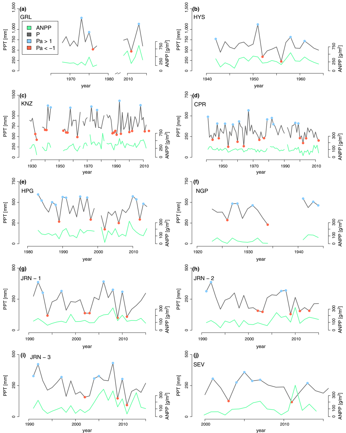
FIGURE 2 Timeseries of water year precipitation [PPT: mm] and aboveground net primary production [ANPP: g/m 2 ] for each grassland site. Water year PPT anomaly [ P_a : (PPT - \overline{PPT})/\sigma_{PPT} ] > 1.0 is indicated by blue dots, and water year P_a < -1.0 is indicated by red dots. JRN data included three grassland sites [Colour figure can be viewed at wileyonlinelibrary.com ]
