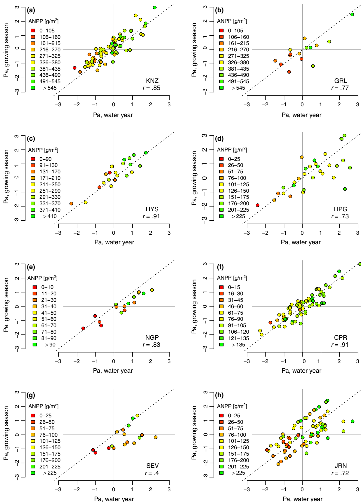
FIGURE 5 Aboveground net primary productivity [ANPP: \text{g/m}^2 ] plotted against water year PPT anomaly [ \text{Pa} : (\text{PPT} - \overline{\text{PPT}})/\sigma_{\text{PPT}}^2 ] and growing season Pa for each grassland site. Pearson's r is provided for each site and is based on the 1:1 line. The ANPP scale differs between sites [Colour figure can be viewed at wileyonlinelibrary.com ]
