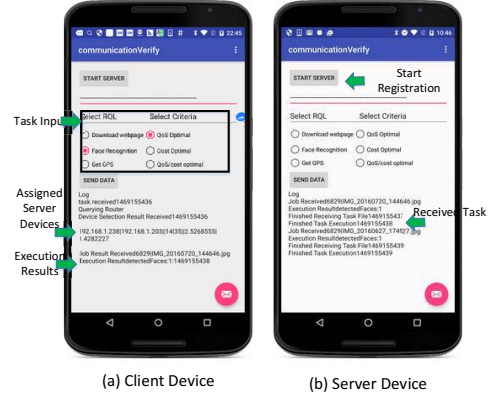
Figure 10: Execution UI.
