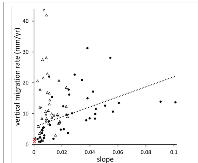
FIGURE 6 | Vertical migration rates of marshes as a function of local slope. Black dots are data collected in Chesapeake Bay (Schieder et al., 2017), triangles in Delaware Bay (Smith, 2013), and red crosses in Florida (Raabe and Stumpf, 2015). The dotted line is the linear interpolation of the Chesapeake Bay data.
