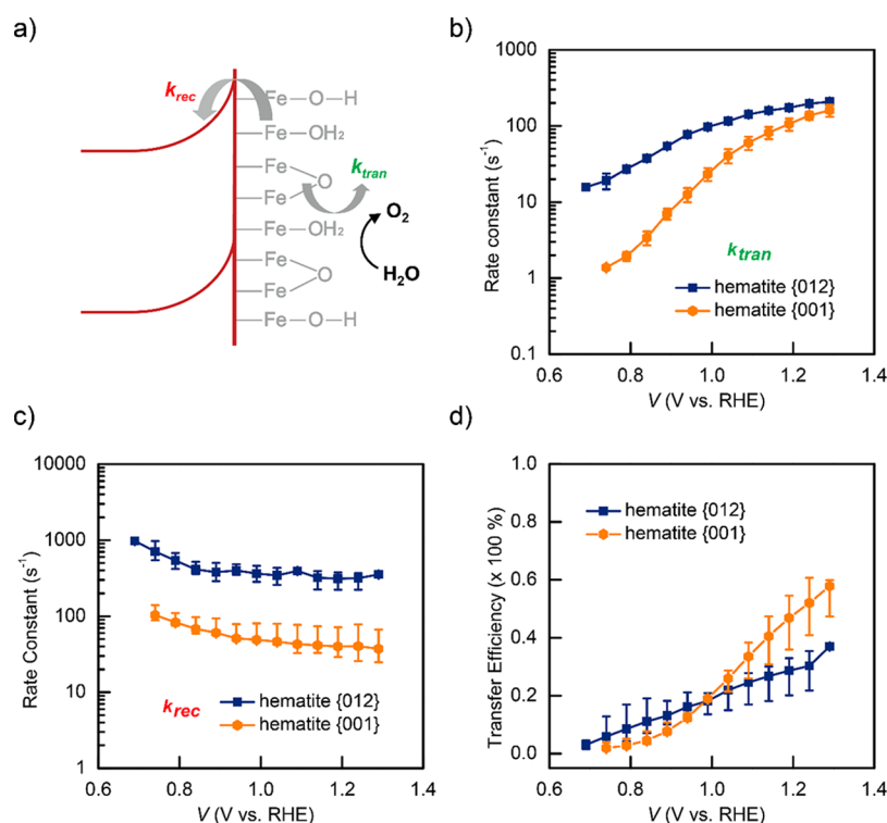
Figure 5. Kinetic comparisons of hematite {012} and hematite {001} . (a) Kinetic model describing the competing charge transfer and recombination processes under PEC water oxidation conditions. It is assumed that water oxidation by hematite is mediated by surface chemisorbed OH species. Comparisons of: (b) rate constant for charge transfer, (c) rate constant for charge recombination, and (d) charge transfer efficiency for hematite {012} and hematite {001} , respectively.
