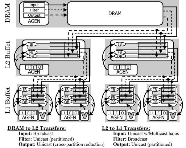
Figure 9. Example accelerator derived from the EDDO in Figure 8 with multiple levels of buffets sharing RAMs. For simplicity, paths for cross-partition reduction of partial sums are not shown.
