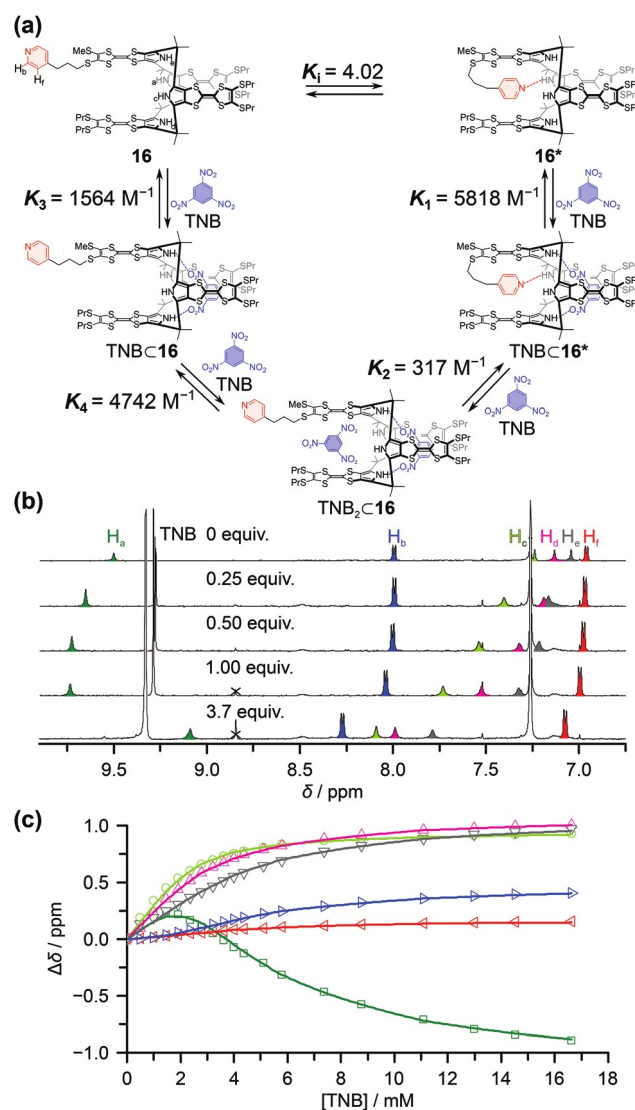
Fig. 25 Interactions of 16 and TNB shown in the form of (a) a mechanistic scheme with associated equilibrium constants as estimated by (b) 1 H NMR spectroscopic (400 MHz, 298 K, CDCl 3 ) titrations of 16* (2.00 mM) with increasing quantities of TNB (0 to 8.3 equiv.) wherein the change in the chemical shift of the aromatic signals (c) related to four pyrrole NH protons and two pyridine proton resonances (symbols) are monitored. The lines indicate best fits to the binding isotherms. Adapted from ref. 65. Copyright 2013 Wiley-VCH Verlag GmbH.
