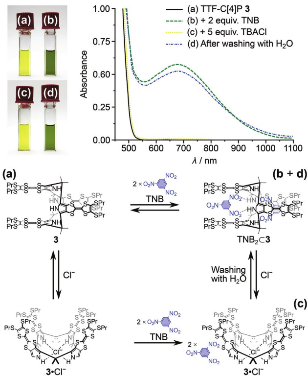
Fig. 5 Top: Absorption spectra ( \text{CH}_2\text{Cl}_2 , 298 K) of (a) 3 (1.0 mM), (b) 3 + two equiv. of TNB, (c) 3 + five equiv. of TBACl and (d) after washing with \text{H}_2\text{O} . Bottom: Equilibrium scheme occurring in the presence and absence of TNB and TBACl as observed by absorption spectroscopy. Adapted from ref. 39. Copyright 2004 American Chemical Society.
