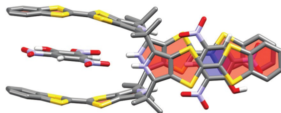
Fig. 14 Single-crystal X-ray structure of the \text{TNB}_2\text{C}_5 complex. All hydrogen atoms except the NH and Ar-H protons have been removed for clarity. 50
