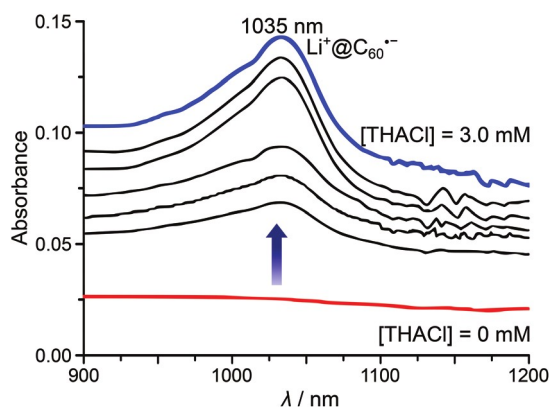
Fig. 30 NIR absorption spectroscopic changes of a solution of equimolar amounts of 3 (50 \mu\text{M} in PhCN at 298 K) and [\text{Li}^+@C_{60}]\text{PF}_6 upon addition of increasing amounts of THACl. Adapted with permission from ref. 68. Copyright 2011 American Chemical Society.
