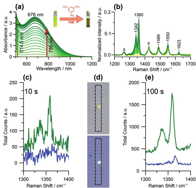
Fig. 17 Solution and solid-state detection of TNB by 3. (a) UV-Vis-NIR absorption spectroscopic titration of 3 (30 mM in \text{CH}_2\text{Cl}_2 at 298 K) with TNB (0–6 equiv.). (b) Resonance Raman spectra of the same titration with excitation at \lambda = 785 nm. (c) and (e) Solid-state resonance Raman spectra ( \lambda_{\text{exc}} = 785 nm) of microcrystalline samples of 3 ((d) top, blue line) and \text{TNB}_2\text{C}_3 ((d) bottom, green line) subject to laser photo-excitation (0.3 mW) for 10 and 100 s, respectively. Adapted from ref. 57 with permission from The Royal Society of Chemistry.
