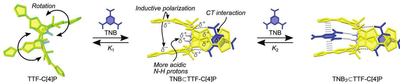
Fig. 15 Schematic representation of the electronically induced effects of TTF-C[4]P that occur upon binding a single electron-deficient planar guest (e.g. TNB). This first recognition event results in a formation of preferentially organised 1,3-alternate conformation. It also increases the acidity of the free (i.e. uncomplexed) NH protons and enhances the electron density of the uncomplexed TTF-C[4]Ps. These effects lead to a cooperative binding mode where K_2 \gg K_1 . 41,50
