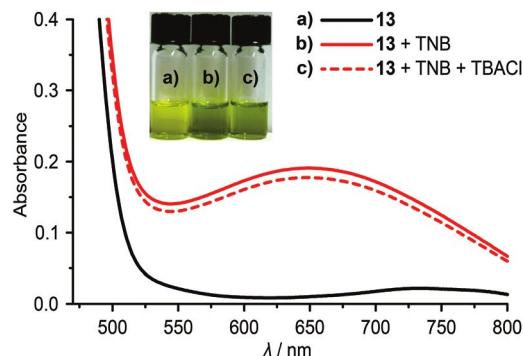
Fig. 21 UV-Vis absorption spectroscopic titration ( CH_2Cl_2 , 298 K) of 13 with addition of five equiv. of TNB and subsequent addition of ten equiv. of TBACl. Insert of the solutions during titration. Adapted with permission from ref. 59. Copyright 2009 Springer.
