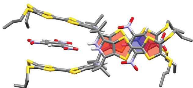
Fig. 4 Crystal structure of the \text{TNB}_2\text{C}_3 complex. All hydrogen atoms except the NH and Ar-H protons have been removed for clarity. 39
