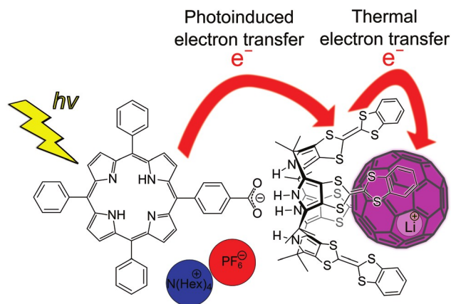
Fig. 33 Complex \text{Li}^+@C_{60} -5·19 formed when the counter cation (in blue) is \text{THA}^+ . In this ensemble permits both thermal ET between 5 and \text{Li}^+@C_{60} and PET from the porphyrin (19) to the TTF-C[4]P.
