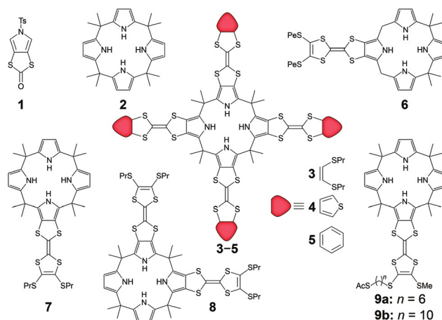
Fig. 1 Chemical structures of TTF-pyrrole precursor 1 , meso-octamethylcalix[4]pyrrole 2 , tetrakis-TTF-calix[4]pyrroles 3–5 , mono-TTF-calix[4]pyrroles 6 and 7 , bis-TTF-calix[4]pyrrole 8 and thioacetyl mono-TTF-calix[4]pyrroles 9a–b .
