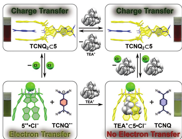
Fig. 35 Illustration of the ionically controlled supramolecular tristate switching operation controlled by the selective addition of cation ( \text{TEA}^+ ) and anion ( \text{Cl}^- ) pairs to stabilise three limiting states, involving charge transfer (“Hi-Z” state), ET (“1” state) or no ET (“0” state), respectively. Adapted with permission from ref. 71. Copyright 2018 American Chemical Society.
