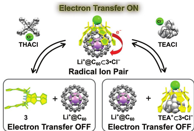
Fig. 29 Illustration of the ion-controlled ON-OFF switching of ET from 3 to \text{Li}^+@C_{60} . Upon addition of THACl to a mixture of 3 and \text{Li}^+@C_{60} a favourable cone-conformation of 3\cdot\text{Cl}^- is formed allowing for the capture of \text{Li}^+@C_{60} within the cavity. Addition of TEACl to this complex instigates a competition between \text{TEA}^+ and \text{Li}^+@C_{60} for the cavity of 3\cdot\text{Cl}^- thereby turning off the ET process.
