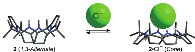
Fig. 2 Change in the dominant conformation seen upon the binding of a chloride anion to meso-octamethyl-calix[4]pyrrole 2.
