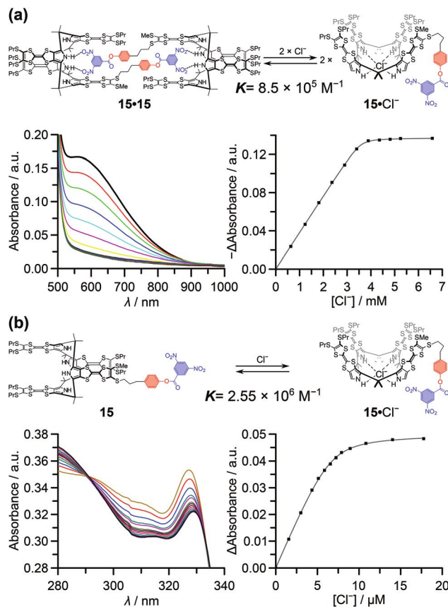
Fig. 24 UV-Vis-NIR absorption spectroscopic titrations (CH 2 Cl 2 , 298 K) of 15 with TBACl carried out at two different concentrations of 15 : (a) at high concentration (0.4 mM) the dimer 15·15 is the dominant species. (b) At low concentration (6.6 μM) the monomer 15 is the predominant species in solution, resulting in a higher apparent complexation constant for chloride anion binding. Adapted from ref. 64. Copyright 2012, with permission from Elsevier.
