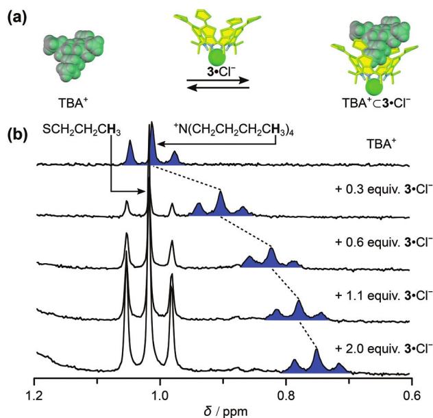
Fig. 8 Complexation of TBA + with 3·Cl - : (a) Scheme illustrating the complexation event and (b) partial 1 H NMR spectra (CDCl 3 , 200 MHz) seen upon the addition of TBAPF 6 to a mixture of 3 and excess KCl containing six equiv. of dicyclohexano-18 crown-6. This process generates 3·Cl - as the initial receptor-containing species. Adapted from ref. 47. Copyright 2008, with permission from Elsevier.
