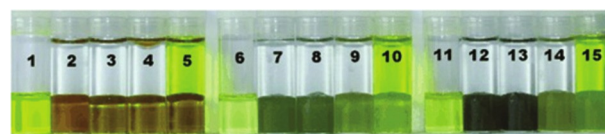
Fig. 16 Colourimetric sensing of TNB, TNT and TNP using receptors 3–5 (2 mL of 0.2 mM in CHCl 3 ) and test nitroaromatic explosives TNB, TNT and TNP (3 mL of 0.2 mM in H 2 O) in the absence and presence of salts (2 mM of NaHCO 3 , K 2 CO 3 , MgSO 4 , CaCl 2 and NH 4 Cl each). Vials from the left contain: (1) 3, (2) 3 + TNB, (3) 3 + TNB + salts, (4) 3 + TNT, (5) 3 + TNP, (6) 4, (7) 4 + TNB, (8) 4 + TNB + salts, (9) 4 + TNT, (10) 4 + TNP, (11) 5, (12) 5 + TNB, (13) 5 + TNB + salts, (14) 5 + TNT and (15) 5 + TNP. Reprinted from ref. 50. Copyright 2010 Wiley-VCH Verlag GmbH.
