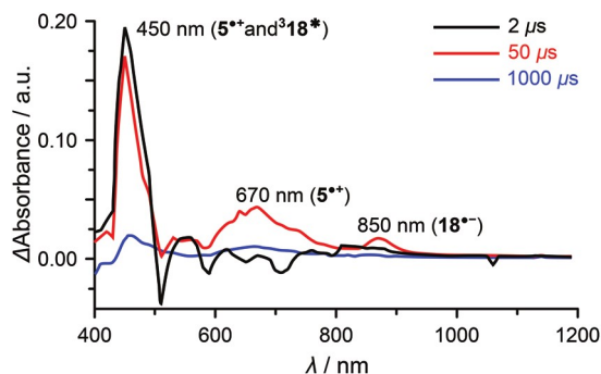
Fig. 32 Nanosecond flash photolysis absorption spectra for a mixture of 5 (0.3 mM) and 18 (0.10 mM) in PhCN at 298 K upon excitation at \lambda = 532 nm. Spectra recorded after 2 \mu\text{s} (black), 50 \mu\text{s} (red) and 1000 \mu\text{s} (blue). Adapted with permission from ref. 69. Copyright 2014 American Chemical Society.
