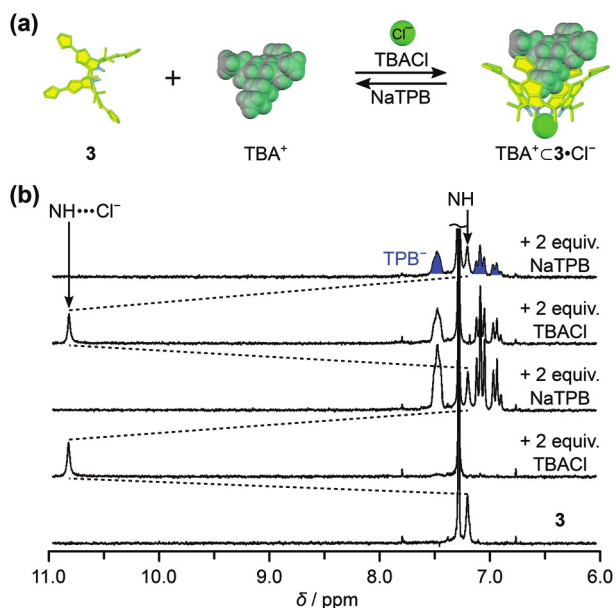
Fig. 9 Complexation of 3 and \text{TBA}^+ in the presence and absence of chloride anion: (a) mechanistic scheme illustrating the complexation event, (b) partial ^1\text{H} NMR spectra ( \text{CDCl}_3 , 200 MHz) of 3 upon stepwise addition of \text{TBACl} and \text{NaTPB} , respectively, showing the complexation and decomplexation of chloride. Adapted from ref. 47. Copyright 2008, with permission from Elsevier.
