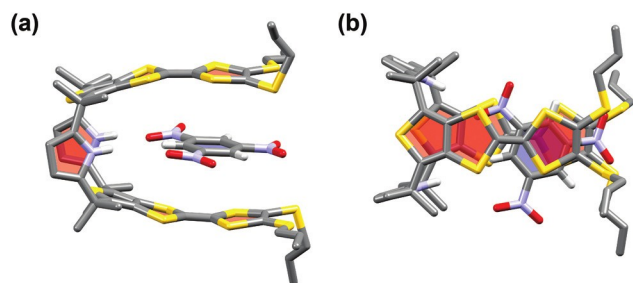
Fig. 20 Single-crystal X-ray structure of the complex TNB \subset 13 obtained by slow diffusion of n -hexane into a CH_2Cl_2 solution containing an equimolar mixture of 13 and TNB. The structure is shown in side (a) and top (b) views. The CH hydrogen atoms on 13 have been removed for clarity. 59
