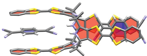
Fig. 34 Single-crystal X-ray structure of the complex \text{TCNQ}_2 \cdot 5 obtained by slow evaporation of a 1 : 2 \text{CH}_3\text{Cl} solution of 5 and TCNQ, respectively. \text{CH}_3\text{Cl} and \text{CH} hydrogens on 5 have been removed for clarity. 71
