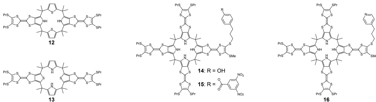
Fig. 18 Chemical structures of modified TTF-C[4]Ps 12–16.
