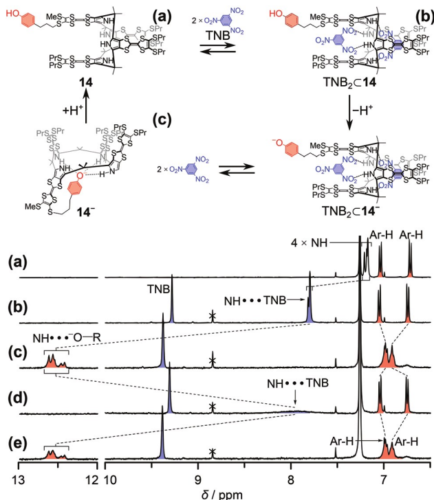
Fig. 22 Schematic illustration (top) of the molecular recognition events that are seen for 14 with TNB in the presence of acid and base and partial 1 H NMR spectra (400 MHz, 298 K, CDCl 3 ) of (a) receptor 14 (1.5 mM), (b) 14 + two equiv. TNB, (c) 14 + two equiv. TNB + one equiv. DBU, (d) 14 + two equiv. TNB + one equiv. DBU + one equiv. MSA and (e) 14 + two equiv. TNB + one equiv. DBU + one equiv. MSA + one equiv. DBU. Adapted from ref. 60. Copyright 2011 Wiley-VCH Verlag GmbH.
