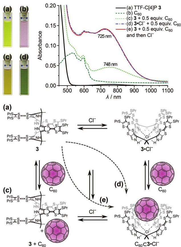
Fig. 6 Top: Absorption spectra (CH 2 Cl 2 , 298 K) of (a) 3 (0.135 mM), (b) C 60 (0.0687 mM), (c) 3 + 0.5 equiv. of C 60 , (d) 3·Cl - + 0.5 equiv. of C 60 and (e) 3 + 0.5 equiv. of C 60 with excess Cl - added. Bottom: Equilibrium scheme occurring in the presence and absence of Cl - and C 60 as observed by absorption spectroscopy. Adapted from ref. 42. Copyright 2006 Wiley-VCH Verlag GmbH.
