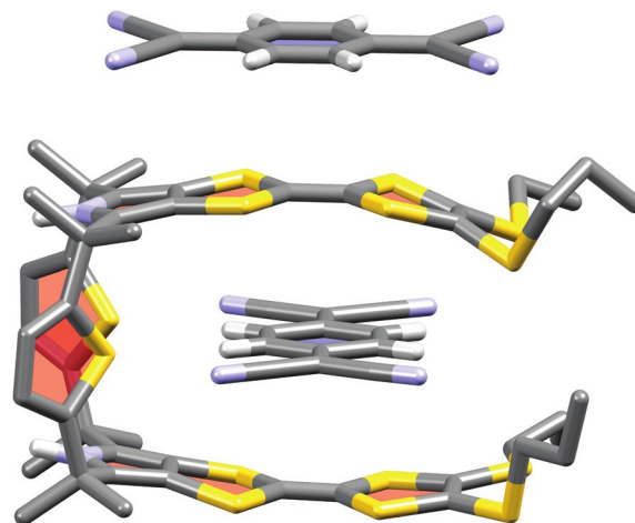
Fig. 19 Single-crystal X-ray structure of the complex \text{TCNQ} \subset 12 \cdot \text{TCNQ} obtained by slow evaporation of a \text{CH}_2\text{Cl}_2 solution of equimolar concentration of 12 and TCNQ. \text{CH}_2\text{Cl}_2 and CH hydrogen atoms on 12 have been removed for clarity. 58
