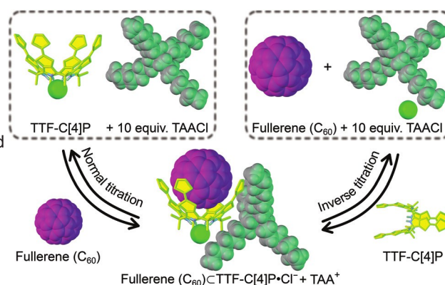
Fig. 11 Illustration of the two titration methods used to probe the interactions between \text{TTF-C}[4]\text{P} and fullerene.
