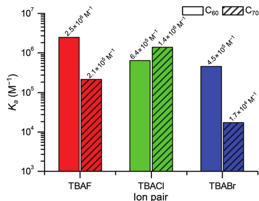
Fig. 10 Estimated binding constants of \text{TBA}^+\text{C}^-\text{X}^- with fullerene based on a normal titration protocol.
