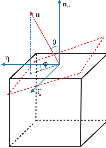
Figure 22. The geometry of facet tilting on a hexahedron. \eta and \zeta are relative coordinates. \theta and \varphi are tilting angles and \varphi rotation is carried out first. \mathbf{n}_0 is the normal vector of the facet before tilting, and \mathbf{n} is the normal vector of the tilted facet.
