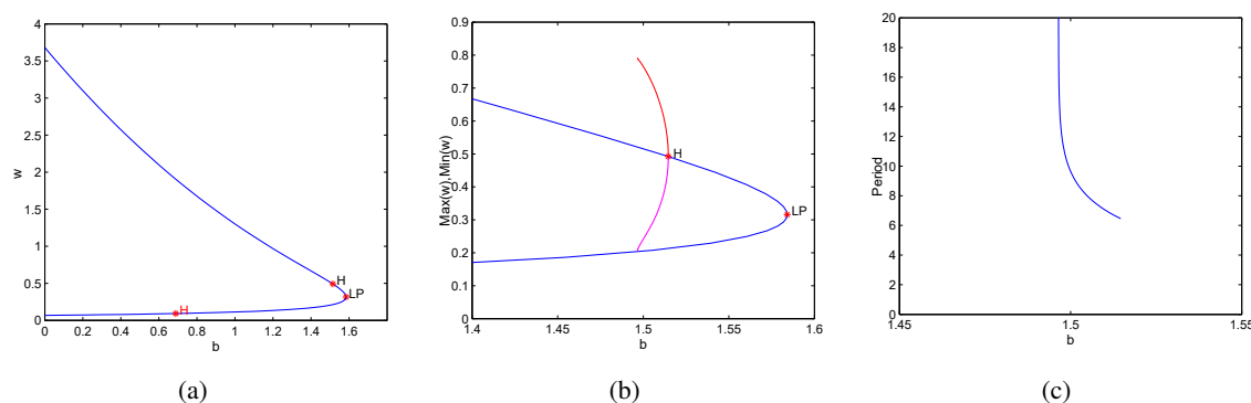
Figure 1. Homoclinic bifurcation, saddle-node bifurcation, subcritical Hopf bifurcation and the existence of one unstable limit cycle when \mu_1 = 1, \mu_2 = 1, \xi_1 = 4, \xi_2 = 0.51, a = 20 . In all diagrams, the horizontal axis is b . The black “H” mark indicates a Hopf bifurcation point; the “LP” mark indicates a saddle-node bifurcation point. (a): Bifurcation diagram. (b): The maximum and the minimum of the cycles. (c): Periods of the stable periodic orbits.
