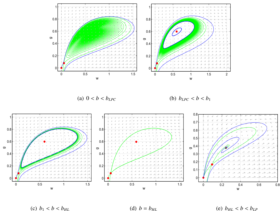
Figure 6. Evolution of phase portraits of (1.2) for \mu_1 = 1, \mu_2 = 2, \xi_1 = 11, \xi_2 = 0.95, a = 52 . (a) b = 3.12 ; (b) b = 3.13 ; (c) b = 3.14 ; (d) b = 3.1562665 ; (e) b = 4 .
