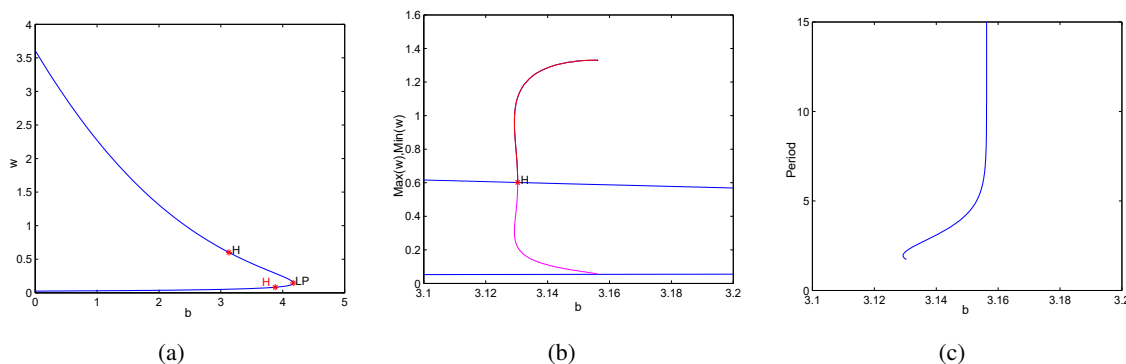
Figure 5. Homoclinic bifurcation, saddle-node bifurcation, subcritical Hopf bifurcation and the existence of two limit cycles when \mu_1 = 1, \mu_2 = 2, \xi_1 = 11, \xi_2 = 0.95, a = 52 . In all diagrams, the horizontal axis is B . The black “H” mark indicates a Hopf bifurcation point; the “LP” mark indicates a saddle-node bifurcation point; and the red “H” mark is a neutral saddle point which is not a bifurcation point. (a): Bifurcation diagram. (b): The maximum and the minimum of the cycles. (c): Period of the stable periodic orbits.
