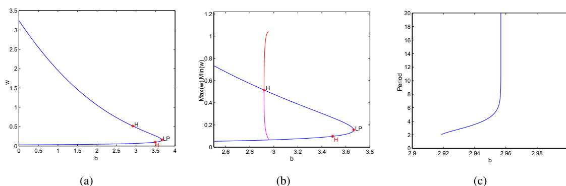
Figure 3. Homoclinic bifurcation, saddle-node bifurcation, supercritical Hopf bifurcation and the existence of one stable limit cycle when \mu_1 = 1, \mu_2 = 2, \xi_1 = 11, \xi_2 = 0.95, a = 48 . In all diagrams, the horizontal axis is b . The black “H” mark indicates a Hopf bifurcation point; the “LP” mark indicates a saddle-node bifurcation point; and the red “H” mark is a neutral saddle point which is not a bifurcation point. (a): Bifurcation diagram. (b): The maximum and the minimum of the cycles. (c): Period of the stable periodic orbits.
