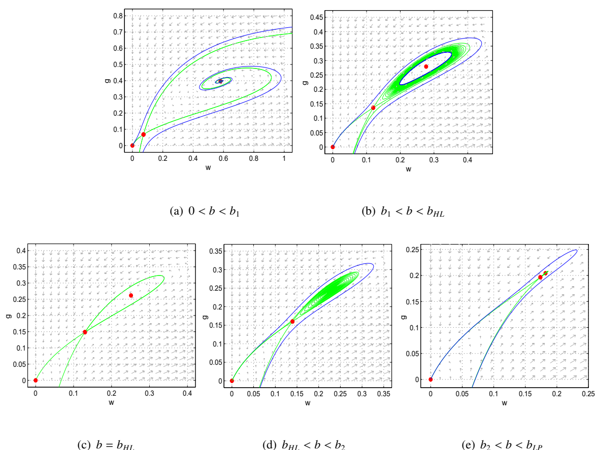
Figure 8. Evolution of phase portraits of (2.1) for \mu_1 = 1, \mu_2 = 2, \xi_1 = 11, \xi_2 = 0.95, a = 40 . (a) b = 2 ; (b) b = 2.55 ; (c) b = 2.59096 ; (d) b = 2.62 ; (e) b = 2.659 .
