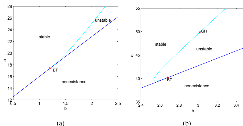
Figure 9. The blue curve represents the saddle-node bifurcation curve and the cyan curve represents the Hopf bifurcation curve. The “BT” mark indicates a Bogdanov-Takens bifurcation point and the “GH” mark indicates a generalized Hopf point where the first Lyapunov coefficient vanishes while the second Lyapunov coefficient does not vanish, which indicates that it is nondegenerate, i.e. Hopf bifurcation changes from subcritical to supercritical. Parameters: (a) \mu_1 = 1, \mu_2 = 1, \xi_1 = 4, \xi_2 = 0.51 ; (b) \mu_1 = 1, \mu_2 = 2, \xi_1 = 11, \xi_2 = 0.95 .
