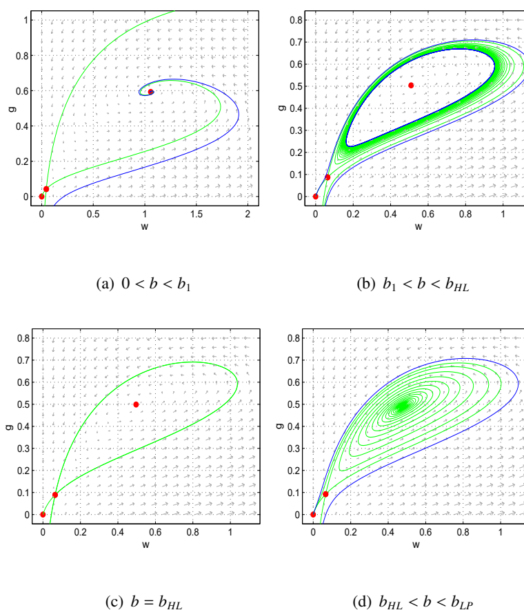
Figure 4. Evolution of phase portraits of (1.2) for \mu_1 = 1, \mu_2 = 2, \xi_1 = 11, \xi_2 = 0.95, a = 48 . (a) b = 2 ; (b) b = 2.93 ; (c) b = 2.9568 ; (d) b = 3 .
