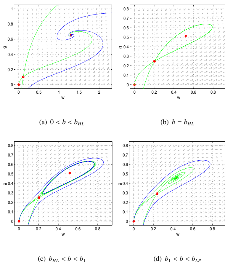
Figure 2. Evolution of phase portraits of (1.2) for \mu_1 = 1, \mu_2 = 1, \xi_1 = 4, \xi_2 = 0.51, a = 20 . (a) b = 1 ; (b) b = 1.4964786 ; (c) b = 1.5 ; (d) b = 1.55 .
