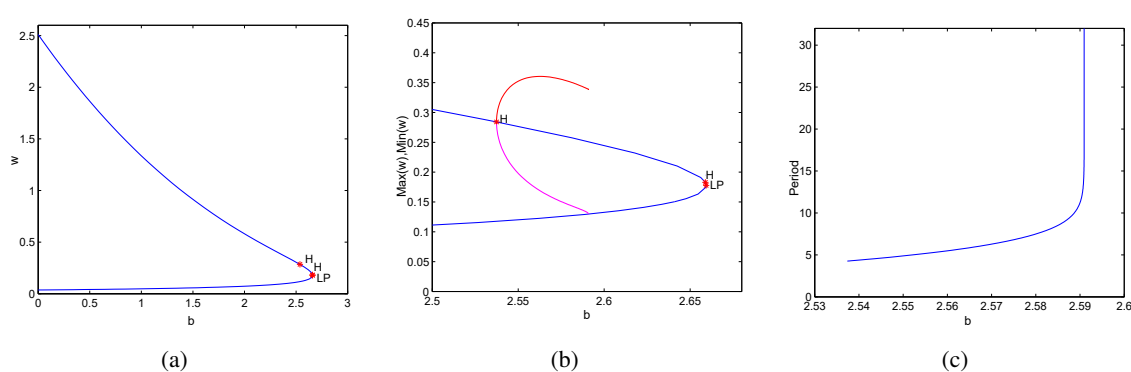
Figure 7. Homoclinic bifurcation, saddle-node bifurcation, two supercritical Hopf bifurcations and the existence of one stable limit cycle when \mu_1 = 1, \mu_2 = 2, \xi_1 = 11, \xi_2 = 0.95, a = 40 . In all diagrams, the horizontal axis is b . The black “H” mark indicates a Hopf bifurcation point; the “LP” mark indicates a saddle-node bifurcation point. (a): Bifurcation diagram. (b): The maximum and the minimum of the cycles. (c): Period of the stable periodic orbits.
