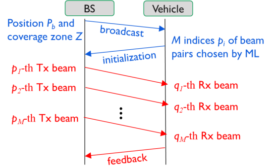
Fig. 1. Timing diagram for the distributed LIDAR-based beam-selection method. The first phase (broadcast and initialization) uses a low-frequency CC while the second corresponds to mmWave communication.
