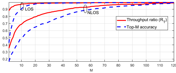
Fig. 5. LOS and NLOS top- M classification for beam-selection with 240 beam pairs in noisy condition for M = 1, \dots, 120 .
