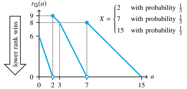
The rank function of the Gittins policy when each job is equally likely to be size 2, 7, or 15. For each age a , the rank function specifies the rank r_G(a) assigned to jobs of age a . The scheduler always serves the job of minimum rank, so we set r_G(a) to be the reciprocal of the job’s Gittins index at age a .
