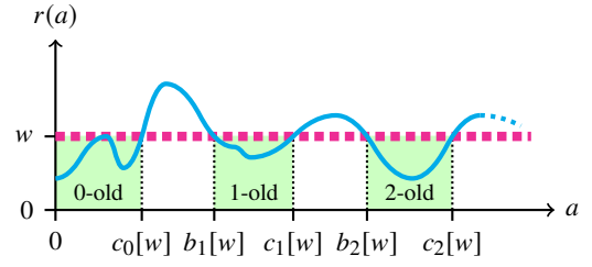
Fig. 7. Illustration of i -Old w -Intervals (Definition 5)
