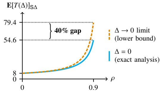
Fig. 5. Response Time of the Shift Gittins Policy
