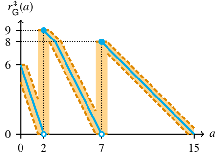
The rank function (blue line), the lower and upper rank functions (lower and upper dashed orange lines, respectively), and the rank bubble function r_G^* (orange region) of the naive Gittins policy when each job is equally likely to be size 2, 7, or 15. The system noise is \Delta = 1/2 .
