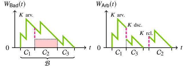
The potential old work (green line) in the Bad (left) and Arb (right) systems. Job K is the second job to arrive in the pictured time ( K arv.). If Arb discards K , the potential old work jumps down (magenta dashed line at K disc.) but later jumps back up the same amount when K is recycled (magenta dashed line at K rel.). This decreases potential old work during C_2 (red region on left is absent on right).
