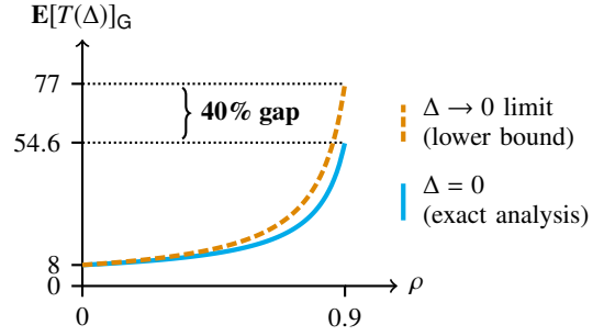
Fig. 3. Response Time of the Naive Gittins Policy
