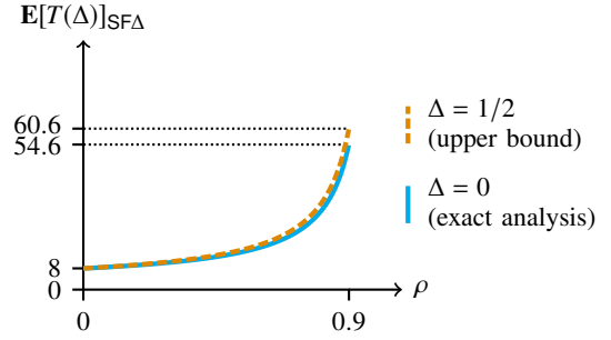
Fig. 6. Response Time of the Shift-Flat Gittins Policy
