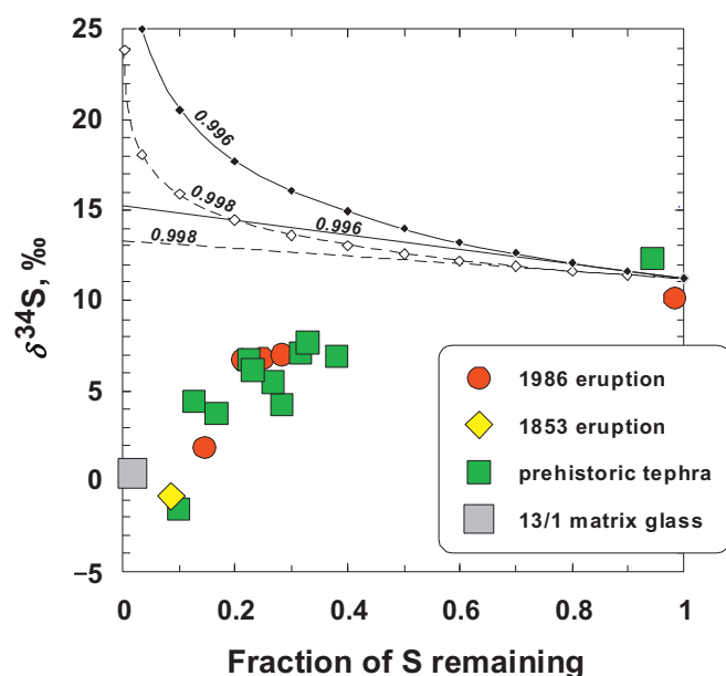
Fig. 9. Sulphur isotope fractionation during magma degassing. The \delta^{34}\text{S} values in the melt inclusions are shown versus fraction of S remaining ( F ). Shifts of \delta^{34}\text{S} were calculated assuming closed-system (equilibrium, solid and dashed straight lines) and open-system (Rayleigh distillation; solid and dashed curves) degassing (see text), the \alpha_{\text{gas-melt}} values of 0.996 and 0.998, and maximum, undegassed S concentration found in the most S-rich melt inclusions having the highest \delta^{34}\text{S} values. At the temperature range from 910 to 1180 °C and the redox conditions of NNO + 1 to NNO + 2 obtained for the studied Chikurachki magmas, the outgassed \text{SO}_2 will drive out the lighter ^{32}\text{S} isotope so that the remaining melt will be progressively enriched in ^{34}\text{S} . Thus, degassing alone cannot explain the observed, \sim 10\% -S-isotope of the studied melt inclusions.
