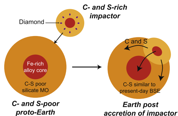
Fig. 9. A schematic diagram illustrating the merger of a C- and S-bearing impacting body to a volatile-free proto-Earth or a proto-Earth whose silicate fraction is C and S-free assuming a simple two-stage core formation. We assume that equilibration was achieved in magma oceans of both the impactor and proto-Earth. We also postulated that the mantle and core of the impactor were directly merged with the mantle and core of the proto-Earth, respectively with minimal interaction between metals and silicates post impact. This cartoon shows that the silicate MO of the impactor would be carbon-rich (graphite or diamond being expelled from the core) owing to the carbon saturation in the S-rich alloy liquid.
