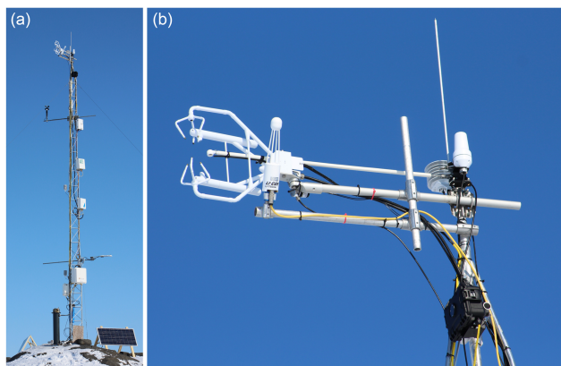
Figure 2. Photograph of the tower (a) and the flux instruments mounted at the top of the tower (b).
