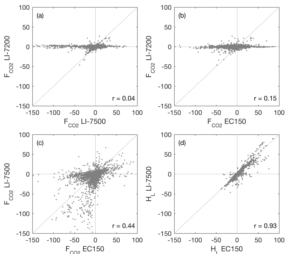
Figure 10. Comparisons of F_{\text{CO}_2} and H_L from the three IRGAs: panel (a) shows F_{\text{CO}_2} (LI-7200) vs. F_{\text{CO}_2} (LI-7500), panel (b) shows F_{\text{CO}_2} (LI-7200) vs. F_{\text{CO}_2} (EC150), panel (c) shows F_{\text{CO}_2} (LI-7500) vs. F_{\text{CO}_2} (EC150), and panel (d) shows H_L (LI-7500) vs. H_L (EC150). Because the sample air to the LI-7200 was dried, comparisons to H_L (LI-7200) were omitted.
