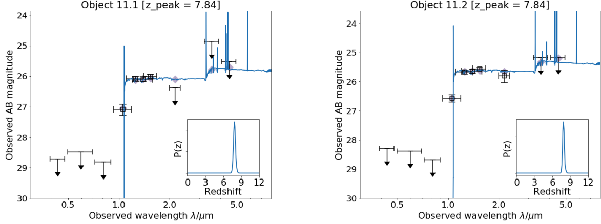
Figure 3. The SEDs and best-fit template for the multiple images in system 11. The IRAC fluxes were extracted from T-PHOT, and the SED fitting was done with the redshift-fitting code EAZY as described in Section 3.1. Error bars and upper limits shown are 1-\sigma . The combined PDFs of the multiple images are shown in Figure 2.
