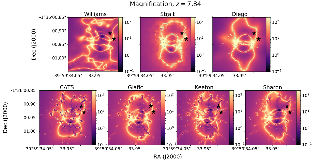
Figure 5. Critical curves at z = 7.84 , the photometric redshift of the images in System 11. Black stars mark the position of the multiple images. The CATS and Sharon groups use lenstool, which uses individual galaxies and other large parameterized mass components. Keeton and Glafic teams are also parametric models, and Diego uses a non-parametric lensing code but a light traces mass assumption. The Williams team along with ours make no such assumptions. All teams but ours used strong lensing constraints only. While shapes of critical curves vary, all groups, including ours (see Figure 1), show good agreement for the images at z = 7.84 .
