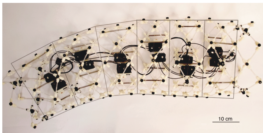
FIG. 12. Overhead view of Compliant Modular Mesh Worm with Steering 20 in a bent configuration. Schematic of six segments projected in the 2D plane is shown. Each segment includes two actuators (black) that change left and right segment side lengths. 2D, two-dimensional.
