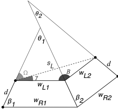
FIG. 8. A pair of trapezoid segments can move together, one elongating and one retracting, without necessitating slip of neighboring segments if the black dots do not move relative to each other. In the text, the geometry of NPWs is calculated from the parameters shown. NPWs, nonperiodic waveforms.
