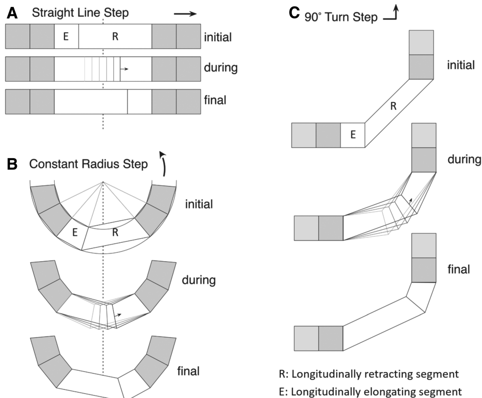
FIG. 4. Balancing a pair of elongating and retracting isosceles trapezoid segments (white) such that the anchoring segments (in gray) do not move. Arrow on top indicates direction of motion. Segments marked R are retracting in length, while segments marked E are elongating in length. A pair of segments retracting and elongating in length are shown for (A) straight-line motion (B) when the body lies along an arc with constant radius, (C) when the posterior and anterior of the body are oriented 90^\circ from each other. The gray segments are anchoring segments and do not move as the retracting and elongating segments change states.
