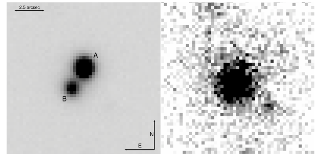
Figure 4. Left: DESJ 0407-5006 Magellan IMACS i image with the naming convention. Right: contrast enhanced (30x) version of the same image with PSFs of the two quasar images subtracted.
