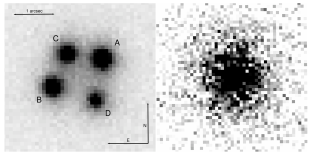
Figure 1. Left: DESJ 0405-3308 SOAR SAMI z image with naming convention. Right: contrast enhanced (10x) version of the same image with PSFs of the four quasar images subtracted.
