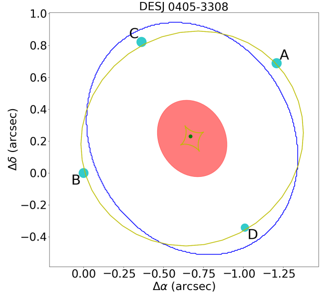
Figure 3. DESJ 0405-3308 lens model. Caustics are shown in yellow and the critical curve in blue. The source quasar is shown in green and the lens galaxy in red.
