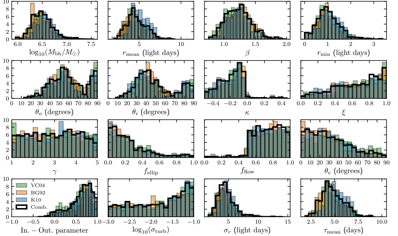
Figure 6. Posterior distributions of the parameters for PG 1310–108. The blue, orange, and green posterior histograms are for the runs using the spectral decompositions using the K10, BG92, and VC04 Fe II templates, respectively. The black line shows the combined posterior PDF.
