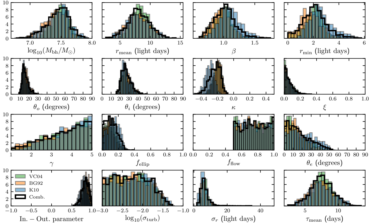
Figure 8. Posterior distributions of the parameters for Mrk 141.
