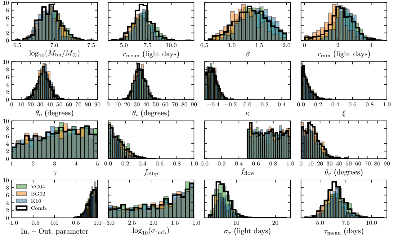
Figure 12. Posterior distributions of the parameters for Zw 229-015.
