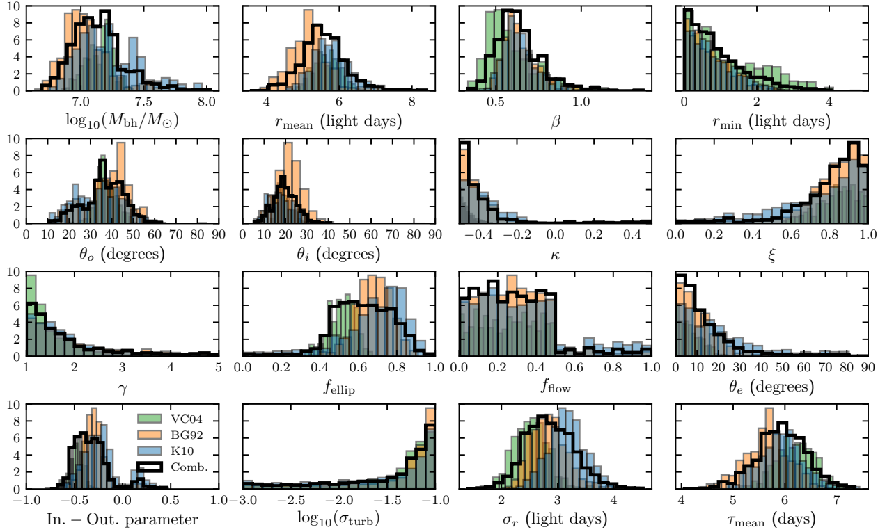
Figure 10. Posterior distributions of the parameters for Mrk 1511.
