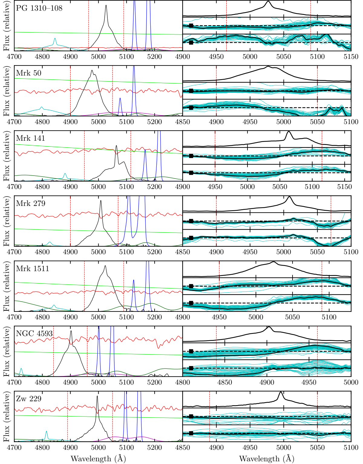
Figure 2. Left: Spectral decomposition using the K10 Fe II template. The components shown are starlight in red, the AGN featureless continuum in lime green, He I in magenta, He II in cyan, [O III] in blue, Fe II in dark green, and the residual H \beta in black. The vertical dashed red lines indicate the wavelength range that was used when fitting the BLR model. Right-top: The mean H \beta profile shape, for reference in the right-middle and right-bottom panels. Right-middle: In black is the mean H \beta spectrum found using the K10 Fe II template minus the mean H \beta spectrum found using the BG92 template. The cyan lines show the same thing, but for every observational epoch. The black bar on the left shows the mean uncertainty in the spectra over the modeled wavelength range. Right-bottom: Same as right-middle, but for the K10 and VC04 templates. For the full spectral decompositions, including the full model fits and residual spectra, see Barth et al. (2015).
