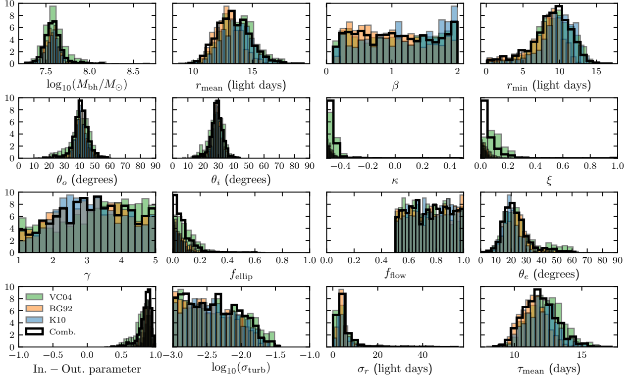
Figure 9. Posterior distributions of the parameters for Mrk 279.
