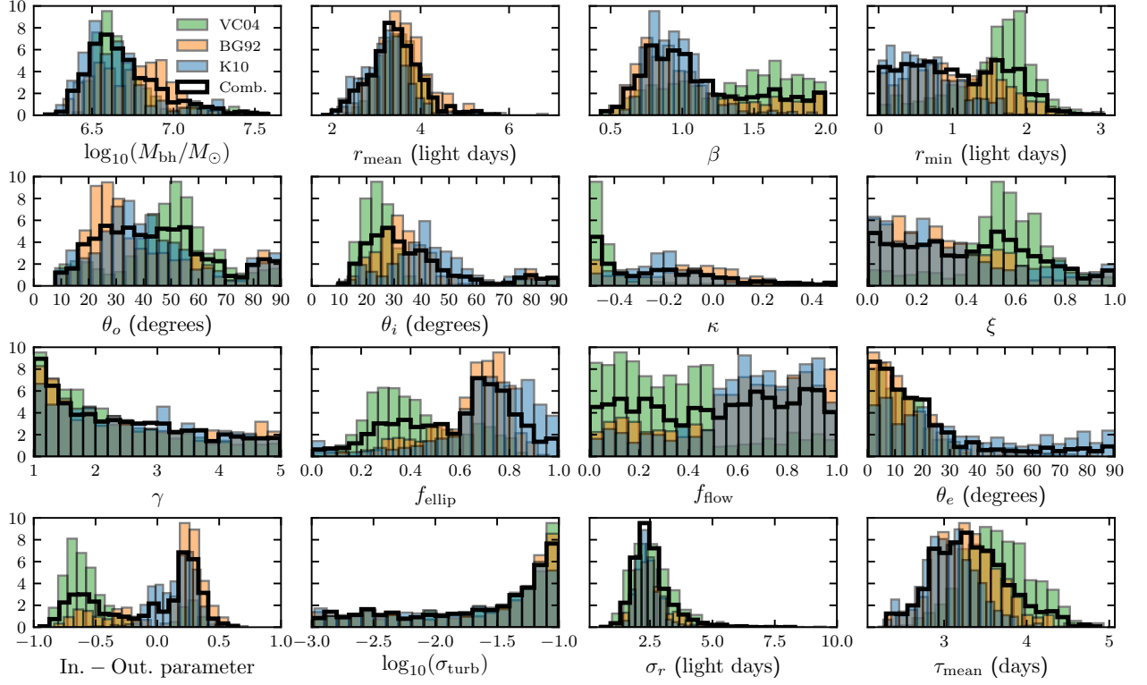
Figure 11. Posterior distributions of the parameters for NGC 4593.
