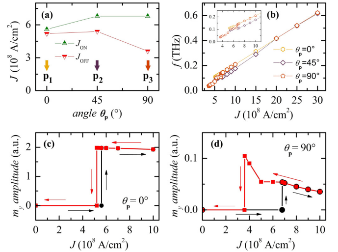
FIG. 2. (a) Threshold current densities ( J_{\text{ON}} and J_{\text{OFF}} ) for the excitation of the antiferromagnetic dynamics for three different directions of spin polarization. (b) Oscillation frequency as a function of the applied current with a zoom near the threshold current. (c), (d) Amplitude of the y component of the magnetization as a function of the current density for \theta_p = 0^\circ and \theta_p = 90^\circ .
