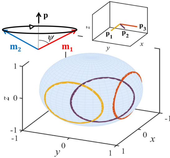
FIG. 3. Trajectories of the magnetizations of the two sublattices in the three different cases of spin Hall polarization, around its direction, for J = 30 \times 10^8 \text{ A/cm}^2 . Left inset: sketch of the precession of the two magnetizations around the spin polarization. Right inset: directions of the spin polarization in the three cases.
