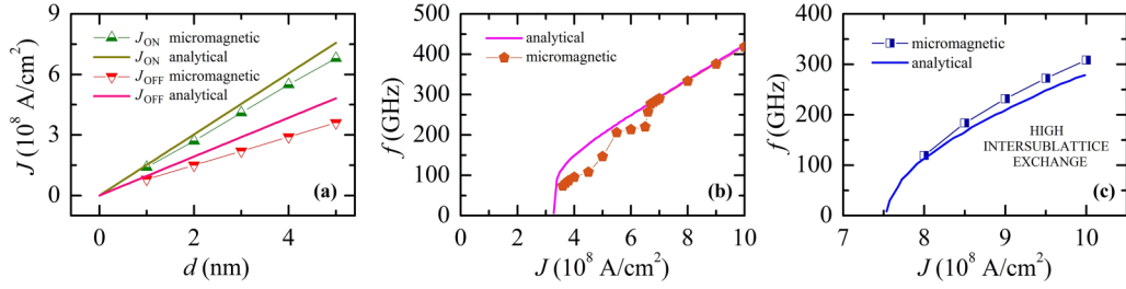
FIG. 5. Comparison between micromagnetic simulations and analytical models in the case \theta_p = 90^\circ : (a) threshold currents, (b) oscillation frequency of the y component of the magnetization, and (c) oscillation frequency of the y component of the magnetization in the case of high intersublattice exchange ( A_{\text{AFM}}/a^2 = 20 \text{ MJ/m}^3 ).
