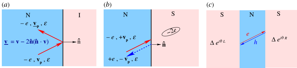
Figure 1. (a) Specular reflection at an N–I boundary, (b) retro-reflection at an N–S boundary and (c) Andreev bound state confined within an S–N–S sandwich. (Online version in colour.)
