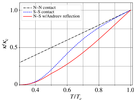
Figure 3. Thermal conductance of an N–N (black dot-dashes), S–S (blue dashes) and N–S (red line) contact. Andreev reflection of quasi-particles for energies above the gap for an N–S contact suppresses the conductance below that of an S–S contact. (Online version in colour.)
