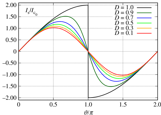
Figure 7. Josephson current-phase relation for an S–c–S point-contact at T = 0 as a function of the transmission probability, 0 < D \leq 1 . The current is normalized by the Ambegaokar–Baratoff critical current at T = 0 , I_c^{AB} = (\pi |\Delta|/2eR_N) \times D . (Online version in colour.)
