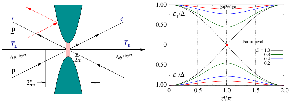
Figure 6. Left: Josephson point contact with radius a \ll \xi_\Delta . Current is transported only via trajectories passing through the aperture with transmission probability D . Right: Branches of Andreev bound states of an S–c–S weak link dispersing as a function of the phase bias, \vartheta . (Online version in colour.)
