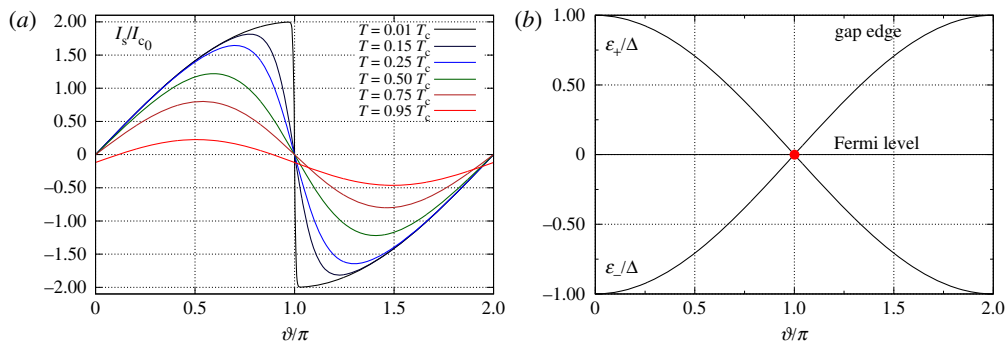
Figure 5. (a) Josephson current as a function of phase bias and temperature for a Sharvin point contact. The current is normalized in units of the Ambegaokar–Baratoff critical current at T = 0 , I_{c0} = \pi \Delta(0)/2e R_N . (b) Branches of Andreev bound states of a Sharvin point contact Josephson weak link dispersing as a function of the phase bias, \vartheta . (Online version in colour.)
