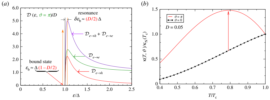
Figure 8. (a) Resonant quasi-particle transmission for an S-c-S Josephson junction tuned to \vartheta = \pi and D = 0.2 . The Andreev bound state lies just below the continuum with \varepsilon_b \simeq |\Delta|(1 - D/2) , giving rise to a transmission resonance at an energy \varepsilon_{\text{res}} \simeq |\Delta|(1 + D/2) . (b) Thermal conductance of a phase-biased S-c-S Josephson weak link. For \vartheta = 0 (black curve), the thermal conductance is suppressed below T_c . For phase bias \vartheta = \pi heat conduction increases sharply below T_c reflecting resonant transmission of hot quasi-particles due to resonant transmission generated by a shallow Andreev bound state [26]. (Online version in colour.)
