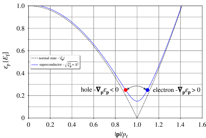
Figure 2. Dispersion relations for the normal state (black dashed line) and superconducting state (solid blue line). Branch conversion scattering is indicated between an electron-like (right blue dot) excitation and a hole-like (left red dot) excitation of the same energy. For illustrative purposes, the excitation gap was set at \Delta = 0.15 E_f . (Online version in colour.)
