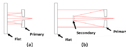
Fig. 10. (a) Alignment of the primary mirror of the Hilbert telescope to the reference 21 in. optical flat. (b) Alignment of the secondary mirror to the primary/flat combination.
