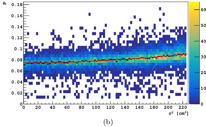
Fig. 5. (a) 2D histogram of T vs. r^2 . The mean values of the bin contents are fit with Eq. (11). The mean values (black points) are under the fit (red curve). (b) 2D histogram of the fast component fraction p vs. r^2 . The mean values of the bin contents are fit with Eq. (12). The mean values (black points) are under the fit (red curve). (See the web version of this article for color.)
