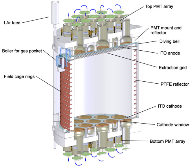
Fig. 1. An illustration of the DarkSide-50 TPC. The height from the bottom fused silica cathode window to the extraction grid is 35.6 cm at room temperature. The LAr surface is slightly above the grid.
