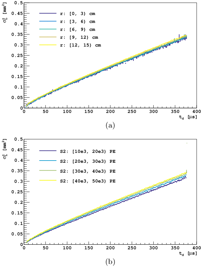
Fig. 11. (a) Diffusion measurement using various r slices with a constant S2 slice. (b) Diffusion measurement using various S2 slices with a constant r slice. (For interpretation of the references to color in this figure legend, the reader is referred to the web version of this article.)
