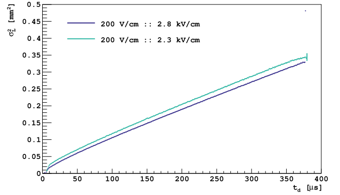
Fig. 13. Mean of \sigma_L^2 vs. t_d for 2.3 kV/cm extraction field data (cyan) and standard 2.8 kV/cm extraction field data (blue). (For interpretation of the references to color in this figure legend, the reader is referred to the web version of this article.)
