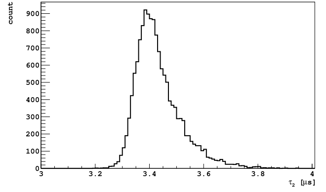
Fig. 6. Distribution of the slow component lifetime \tau_2 , extracted from fits to zero-diffusion events.
