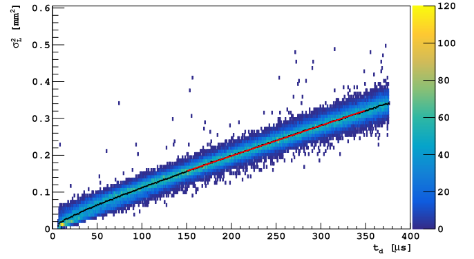
Fig. 10. We extract the Gaussian smearing term \sigma from the S2 pulse shape fits, convert to length scale via \sigma_L = v_d \sigma and plot \sigma_L^2 vs. drift time. The mean of the distribution is black markers and the fit of Eq. (13) to the mean from 50 \mu\text{s} to 350 \mu\text{s} is shown as red curve. (See the web version of this article for color.)
