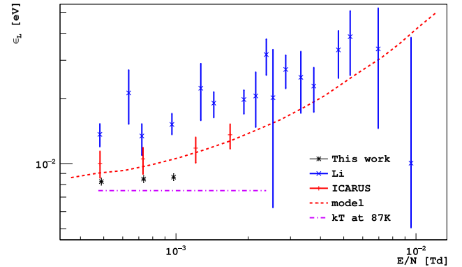
Fig. 16. Electron characteristic longitudinal energy \epsilon_L vs. reduced field ( Td = 10^{-17} V cm 2 ). Li data is from [12] and ICARUS data are extracted from [11]. The model is that of Atrazhev and Timoshkin [21]. The horizontal dashed line represents the thermal energy at 87 K. Error bars are mainly attributable to systematics, including the uncertainty from the nonlinear relation, which is not included in the errors in the other works.
