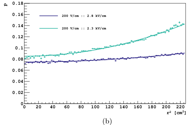
Fig. 12. Mean of (a) T vs. r^2 and (b) p vs. r^2 distributions for standard 2.8 kV/cm extraction field data (blue) and 2.3 kV/cm extraction field data (cyan). (For interpretation of the references to color in this figure legend, the reader is referred to the web version of this article.)
