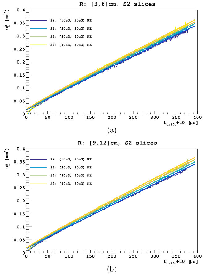
Fig. 14. Simulation results of electron diffusion with self Coulomb repulsion (lines) compared to data from Fig. 11b (points): (a) Events with r = [3, 6] cm, D_L = 3.88 \text{ cm}^2/\text{s} , \sigma_0 = 1.20 \times 10^{-4} \text{ cm}^2 , Y_{S2} = 13.5 \text{ PE/e} . (b) Events with r = [9, 12] cm, D_L = 3.88 \text{ cm}^2/\text{s} , \sigma_0 = 1.20 \times 10^{-4} \text{ cm}^2 , Y_{S2} = 11.5 \text{ PE/e} . Systematic dependence of D_L and \sigma_0 on r can be decoupled by introducing Coulomb repulsion and a r -dependent S2 yield. (For interpretation of the references to color in this figure legend, the reader is referred to the web version of this article.)
