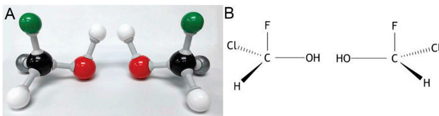
Fig. 1. Physical ball-and-stick model (A) and wedge-dash structure (B). Each shows two molecules with the same atoms but different 3D spatial arrangement of the atoms.
