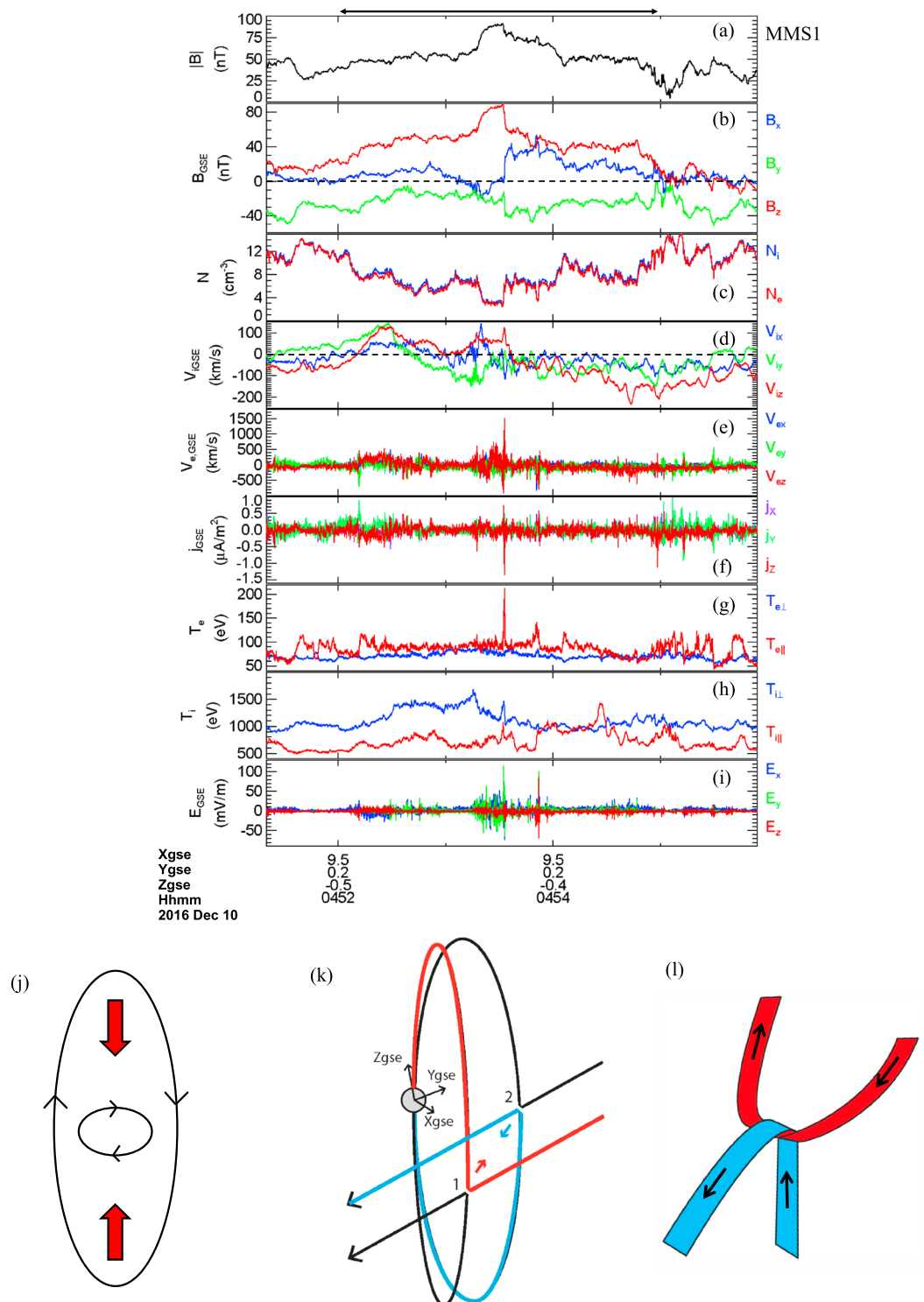
Figure 1. (a–i) MMS1 observations of the large-scale context of the event, in GSE. The interval of enhanced magnetic field and converging jets is marked with the horizontal double arrow. (a, b) Magnetic field magnitude and components, (c) ion and electron densities, (d) ion velocity, (e) electron velocity, (f) current density calculated using plasma data, \mathbf{j} = eN_e(\mathbf{V}_i - \mathbf{V}_e) , (g) electron temperature, (h) ion temperature, (i) electric field. (j) Two-dimensional cartoon illustrating two converging reconnection jets forming closed magnetic loops, a scenario that is inconsistent with the electron pitch angle data (see Figure 2). (k) Three-dimensional sketch showing how nonsimultaneous reconnection at two locations at the magnetopause (first at “1” and then at “2”) can lead to converging plasma jets and interlinked flux tubes. (l) Interlinked flux tubes forming a thin interface current sheet.
