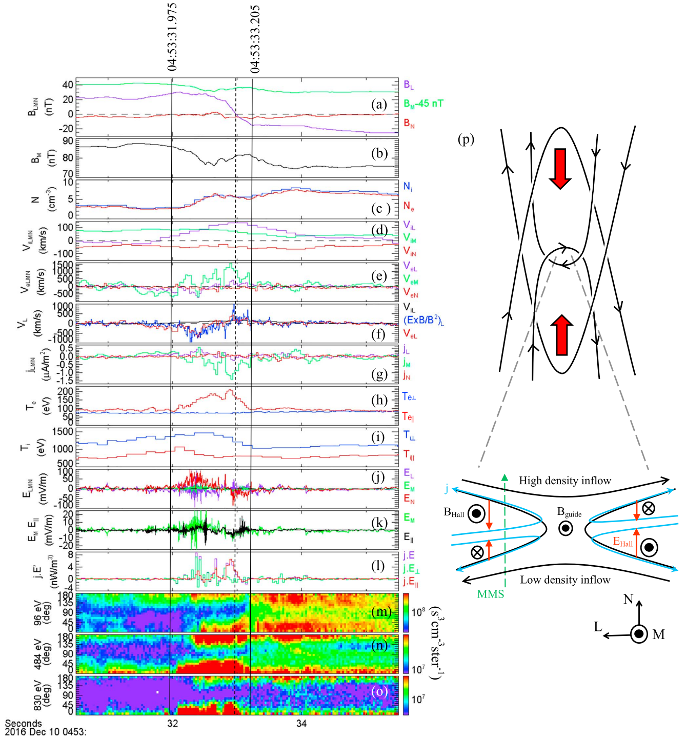
Figure 2. Detailed MMS1 observations of the interface current sheet in LMN, with \mathbf{L} = \text{GSE}(-0.731, 0.530, 0.416) , \mathbf{M} = \text{GSE}(0.253, -0.352, 0.894) , and \mathbf{N} = \text{GSE}(0.628, 0.768, 0.125) . (a) Magnetic field components ( B_M shifted by -45 nT), (b) out-of-plane magnetic field B_M , (c) ion and electron densities, (d) ion velocity, (e) electron velocity, (f) V_{iL} , V_{eL} , and (\mathbf{E} \times \mathbf{B}/B^2)_L , (g) current density \mathbf{j} = eN_e(\mathbf{V}_i - \mathbf{V}_e) , (h) electron temperature, (i) ion temperature, (j) electric field, (k) E_M and E_{||} , (l) \mathbf{j} \cdot \mathbf{E}' = \mathbf{j} \cdot (\mathbf{E} + \mathbf{V}_e \times \mathbf{B}) , (m-o) electron pitch angle spectrograms for 96-, 484-, and 830-eV electrons, (p) conceptual sketch of the 2-D projection of the magnetic field in the interlinked 3-D structure (Figures 1k and 1l) in the L-N plane, with a close-up of the interface current sheet and a possible MMS trajectory. Different energy flux intensities and pitch angle behaviors to the left and right of the current sheet indicate that the two inflow regions are not magnetically connected. The vertical solid lines in (a-o) mark the separatrices (see section S5). The vertical dashed line marks B_L = 0 .
