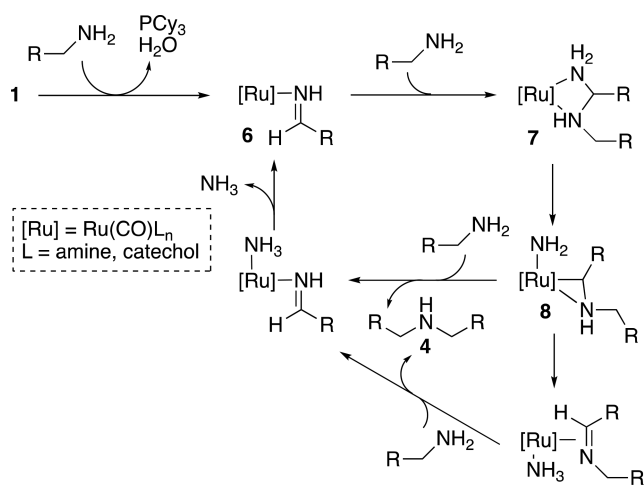
Scheme 1. Proposed Mechanism of the Deaminative Coupling of Primary Amines
