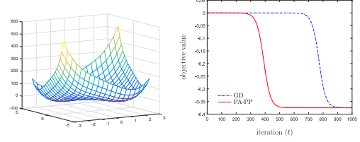
Fig. 1. Convergence comparison between GD and PA-PP, where \epsilon = 10^{-4} , g_{\text{th}} = \epsilon/10 , \nu = 50 , t_{\text{th}} = 10/\epsilon^{1/3} , r = \epsilon/10 .
