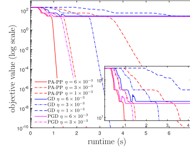
Fig. 2. Convergence comparison among GD, PGD and PA-PP for asymmetric matrix factorization, where \epsilon = 10^{-10} , g_{\text{th}} = \epsilon/10 , t_{\text{th}} = 10/\epsilon^{1/3} , r = \epsilon/10 .
