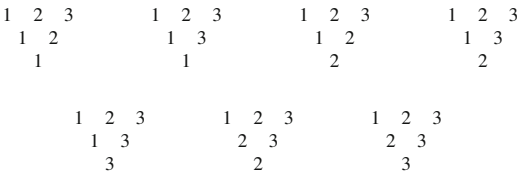
Gog triangles of size 3
