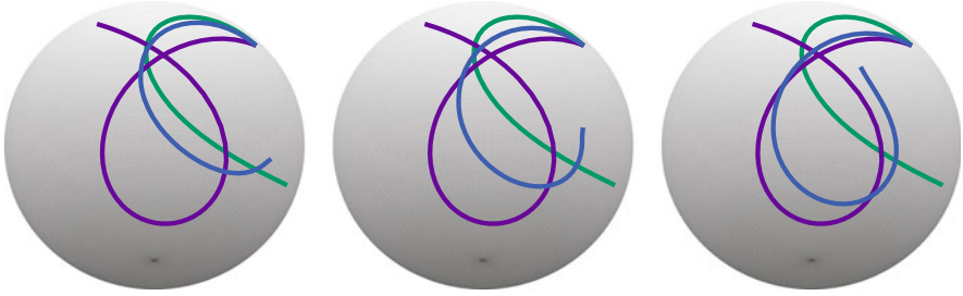
Fig. 1 The blue curve shows the deformation of the green curve into the purple one along a geodesic \gamma: [0, 1] \rightarrow \text{Imm}(I, S^2) plotted for the three times \left\{\frac{1}{4}, \frac{1}{2}, \frac{3}{4}\right\} from left to right
