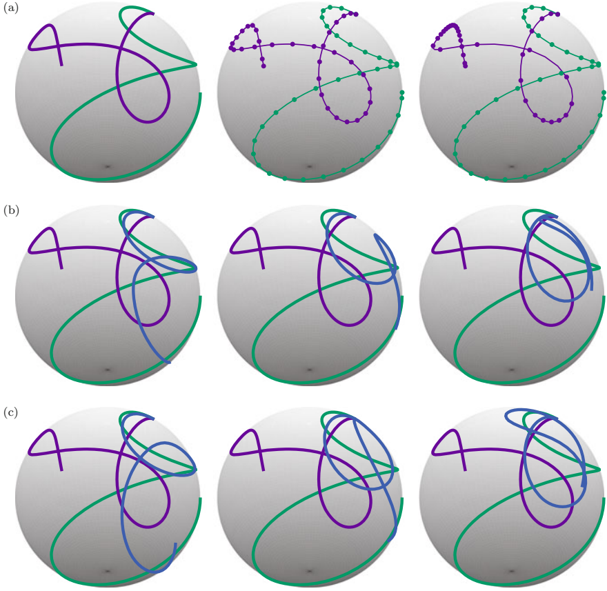
Fig. 3 Interpolation between two curves on S^2 , with and without reparametrisation, found by the reductive SRVT (31). The curves are c^1(t) = R_x(2\pi t)R_y(2\pi t)R_z(\pi t) \cdot (0, 1, 1)^T/\sqrt{2} and c^2(t) = R_z(2\pi t)R_x(2\pi t)R_y(\pi t/2) \cdot (0, 1, 1)^T/\sqrt{2} for t \in [0, 1] , where R_x(t) , R_y(t) and R_z(t) are the rotation matrices in SO(3) corresponding to rotation of an angle t around the x -, y - and z -axis, respectively. (a) From left to right: Two curves on the sphere, their original parametrisations and the reparametrisation minimizing the distance in S^2 , using the reductive SRVT (31). (b) The interpolated curves at times t = \left\{\frac{1}{4}, \frac{1}{2}, \frac{3}{4}\right\} , from left to right, before reparametrisation. (c) The interpolated curves at times t = \left\{\frac{1}{4}, \frac{1}{2}, \frac{3}{4}\right\} , from left to right, after reparametrisation
