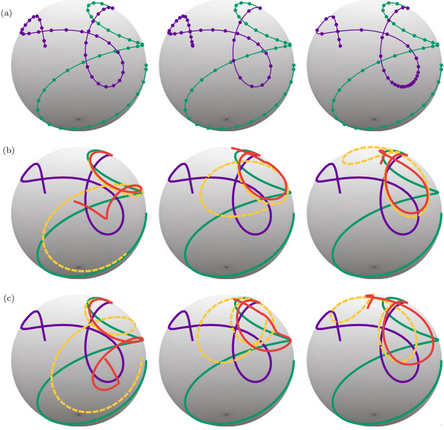
Fig. 4 Interpolation between the same curves as in Fig. 3, with and without reparametrisation, obtained here with the SRVT (30), compared to the corresponding interpolation between curves on \text{SO}(3) mapped to \text{S}^2 by multiplication with the vector (0, 1, 1)^T/\sqrt{2} . (a) From left to right: The original parametrizations of the curves to be interpolated, the reparametrisation minimizing the distance in \text{SO}(3) and the reparametrisation minimizing the distance in \text{S}^2 , using the SRVT (30). (b) The interpolated curves at times t = \left\{\frac{1}{4}, \frac{1}{2}, \frac{3}{4}\right\} , from left to right, before reparametrisation, on \text{SO}(3) (yellow, dashed line) and \text{S}^2 (red, solid line). (c) The interpolated curves at times t = \left\{\frac{1}{4}, \frac{1}{2}, \frac{3}{4}\right\} , from left to right, after reparametrisation, on \text{SO}(3) (yellow, dashed line) and \text{S}^2 (red, solid line)
