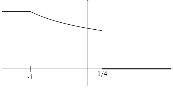
Fig. 2 Limiting density profile, i.e. graph of the function x \mapsto \rho(x, 1)
