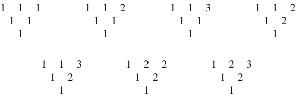
Magog triangles of size 3
