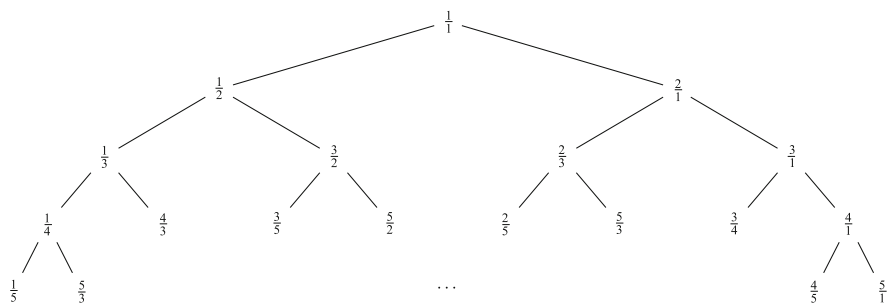
Fig. 8 The Raney tree
