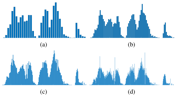
Fig. 9. A comparison of histogram shapes using different numbers of bins: (a) N = 50 , (b) N = 100 , (c) N = 200 , and (d) N = 500 .
