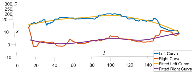
Fig. 8. The results of fitting smooth edges to the leaf using a smoothing spline.
