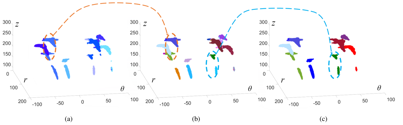
Fig. 5. An example of our clustering results in the space of r , \theta , and z . (a) We use the angle-based clustering to obtain the initial segmentation of the point cloud. However, due to the aliasing problem, the points of two nearby leaves may be clustered together (e.g., the circled blue clusters). (b) We further apply the shape-based clustering to separate these points. (c) We detect and combine the clusters that belong to the same leaf (e.g., the circled green cluster).
