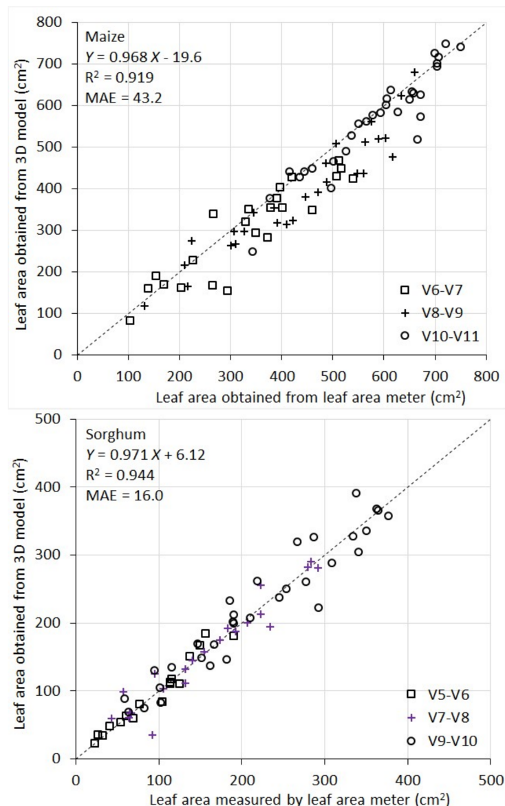
Figure 6. Scatterplot of individual leaf areas of 10 maize and 10 sorghum plants measured by the leaf area meter vs. obtained from 3D plant models. Different legends indicate different growth stages.
