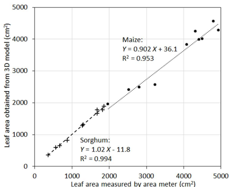
Figure 7. Scatterplot of total leaf areas of the 10 maize plants (circles) and 10 sorghum plants (crosses) measured by the leaf area meter vs. obtained from 3D plant models.
