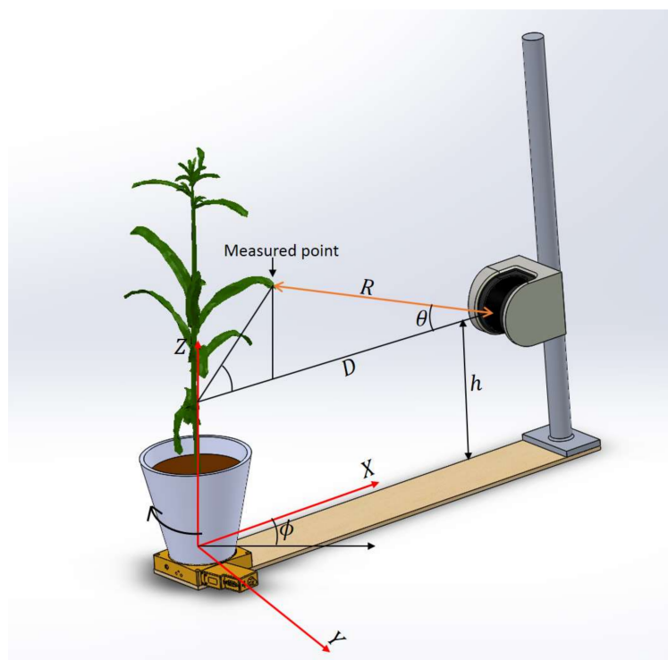
Figure 2. Coordinate system used to convert the range values from the LiDAR to Cartesian coordinates.
