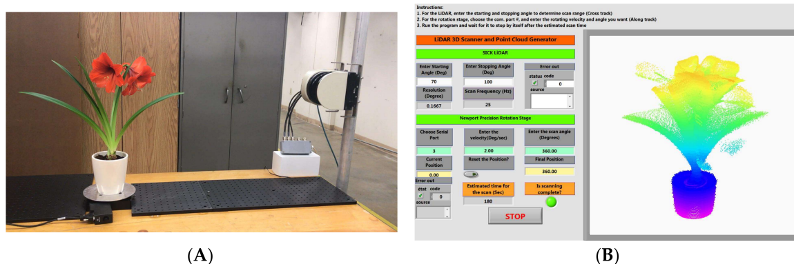
Figure 1. Illustration of the new instrument consisting of a LiDAR scanner and precision rotation stage for 3D measurement of plants at 360° view (A). The LabVIEW graphic user interface for instrument control, measurement acquisition, and real-time point cloud visualization (B).
