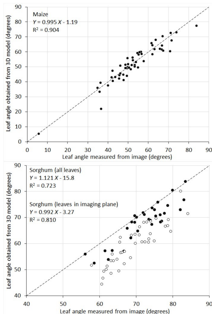
Figure 8. Scatterplot of individual leaf angle of ten maize and ten sorghum plants measured from their RGB images vs. obtained from 3D plant models. For sorghum, solid dots represent the leaves aligned in the imaging plane and hollow dots represent the leaves not in the imaging plane.
