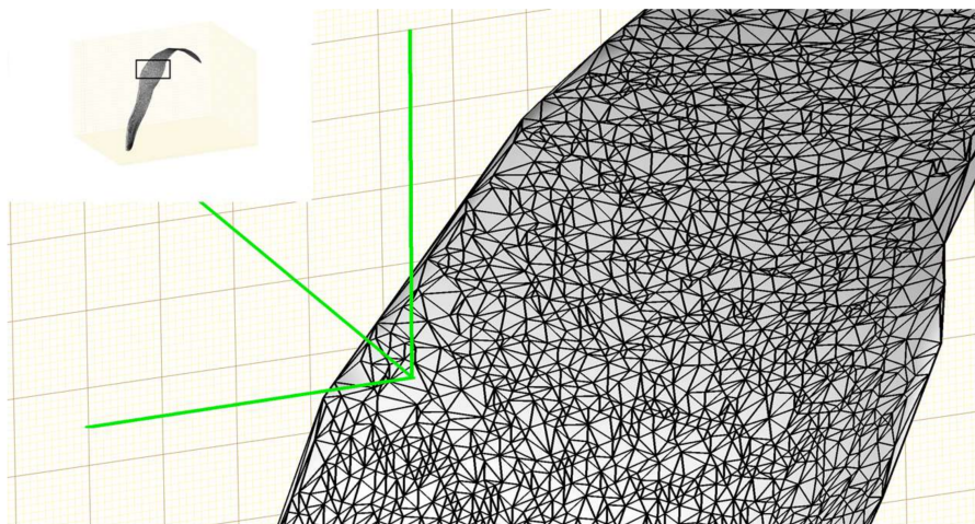
Figure 4. Example of triangulation of a fitted leaf surface in order to calculate leaf area, leaf inclination angle, and leaf angular distribution.
